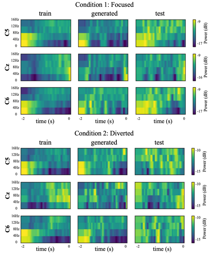
Fig. 7. Average spectrogram of the train, test, and generated samples in MI class. Time 0 shows the movement onset.
