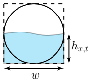
Figure 3: Semi-filled circular pipe approximated with rectangular geometry.
