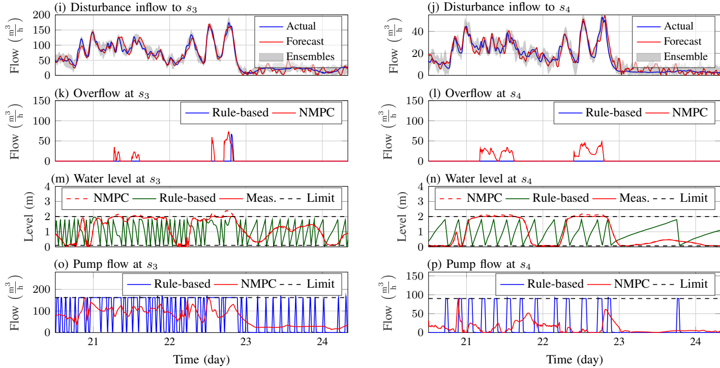
Figure 9-B: NMPC with MHPE and MHSE results compared with rule-based control. (a), (b), (i), (j) show disturbance inflows d_{s,i} , (c), (d), (k), (l) show overflows q_{s,i}^{of} , (e), (f), (m), (n) show states (water levels), while (f), (h), (o), (p) show inputs (pump flows) for each i \in \{1, \dots, N_s\} station, respectively.
