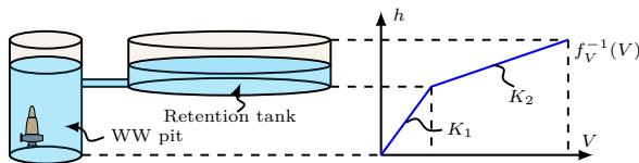
Figure 5: Level-Volume conversion for waste water pit with retention tank.
