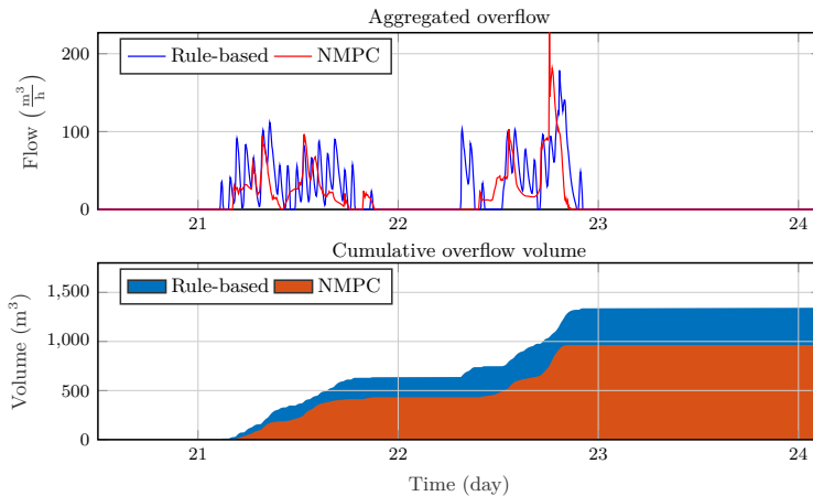
Figure 10: Overflow comparison throughout the entire network.
