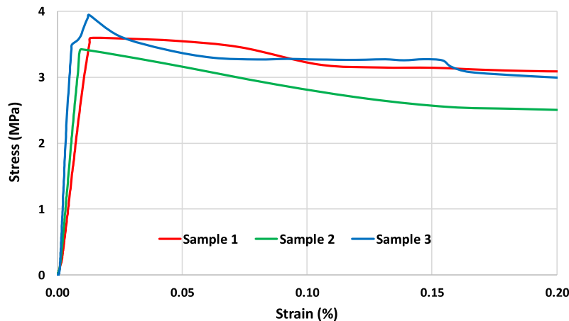
Fig. 2. Tensile stress-strain curve and testing set-up for FRGC specimen.
