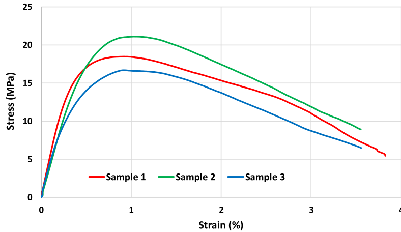
Fig. 1. Compressive stress-strain curve and testing set-up for FRGC specimen.
