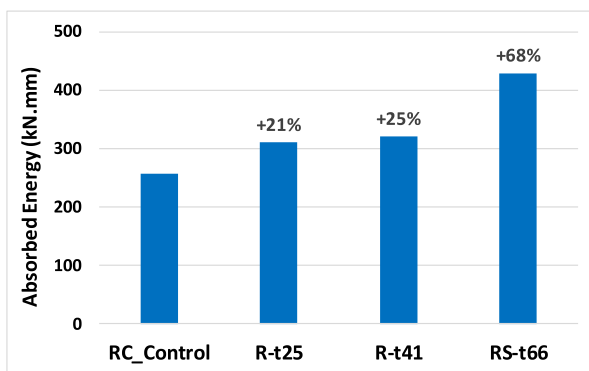
Fig. 12. Energy absorption capacity of repaired beams.
