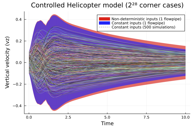
Fig. 6: Reachable states for the vertical velocity of the helicopter model. We consider two cases for the input signals u(t) : constant and non-deterministic. Five hundred trajectories drawn randomly from the set of initial states and with constant inputs are shown on top.
