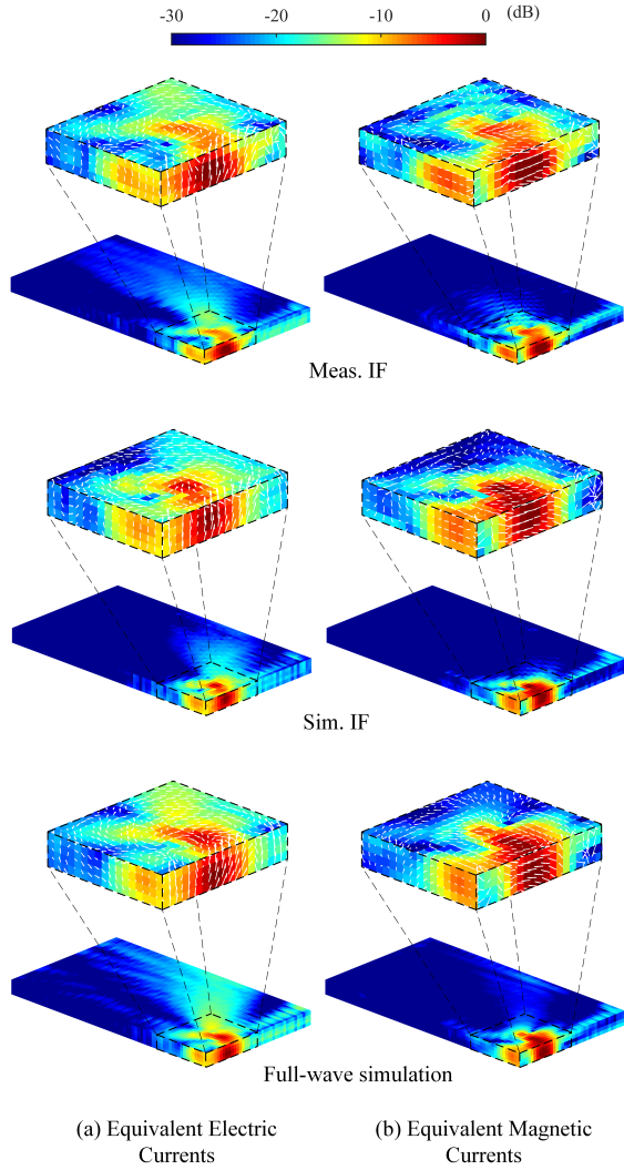
Fig. 17. The normalized EQCs reconstructed from the meas. IF and sim. IF of Ant 1, and those computed from the full-wave simulation at 28 GHz. The left column and the right column are the (a) equivalent electric currents and the (b) equivalent magnetic currents, respectively. The color scale indicates the magnitude of the EQCs, |J_{eq}| and |M_{eq}| . The white arrows in the zoom-in boxes indicate the vector current directions at a particular instant in time, suggesting good agreement of the EQC phases.
