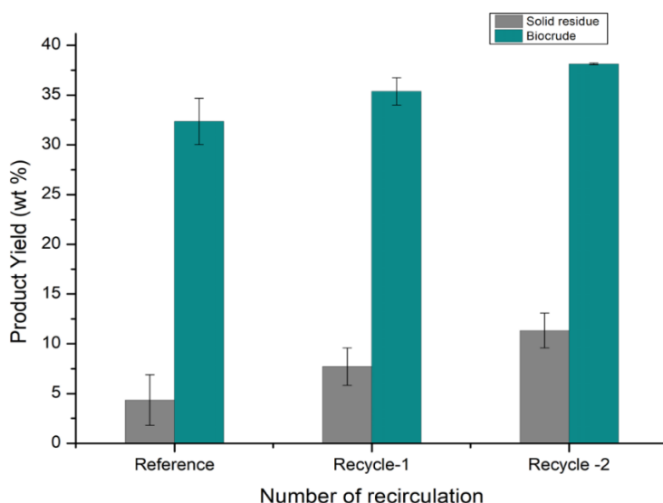
Figure 13: Effect of aqueous phase recirculation on biocrude and solid yield.
