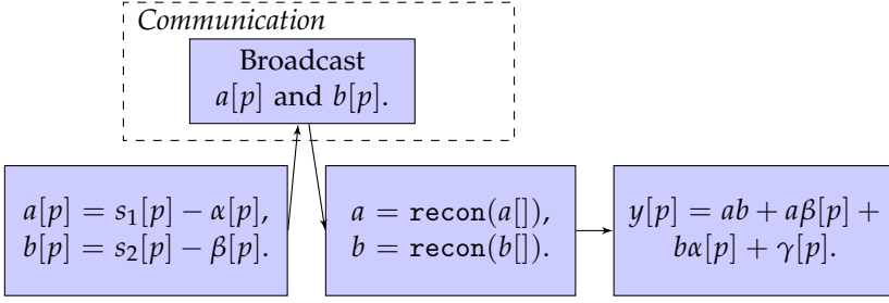
Fig. 10: Block diagram of multiplying two secrets, s_1 and s_2 , using Beavers trick and a Beaver triplet, [\alpha, \beta, \gamma] , from the view of participant p . The product of the secrets is denoted y = s_1 s_2 .
