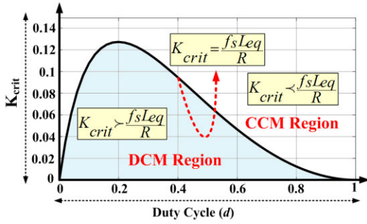
FIGURE 7. CCM and DCM boundary.
