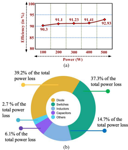
FIGURE 16. Plot (a) Efficiency versus power (b) Power loss distribution of the proposed converter at power 500W and voltage gain 8.
