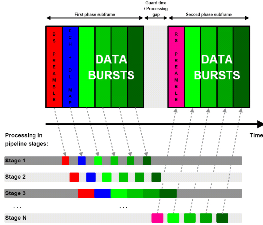
Fig. 5. Pipelined two-hop OFDM(A) frame processing scheme
