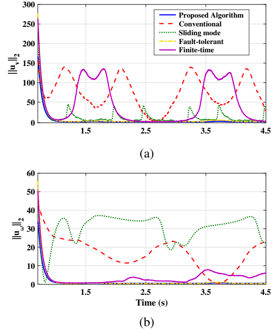
Fig. 8: Comparison of the control efforts of the proposed method with previously reported studies in [14], [11], [19] and, [33]: (a) Voltage and (b) Frequency.
