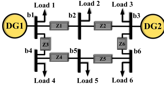
Fig. 6. Studied microgrid structure.
