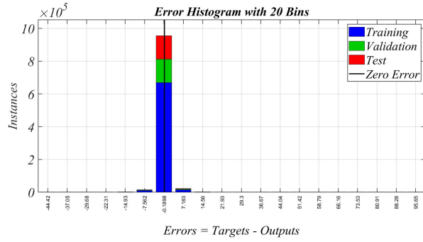
Fig. 5. Error histogram of the ANN with 20 bins. Targets are the real data and the outputs are the outputs of the ANN.
