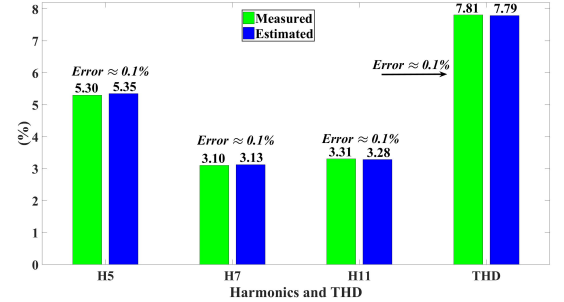
(b) Measured and estimated THD of phase a at desired bus.
