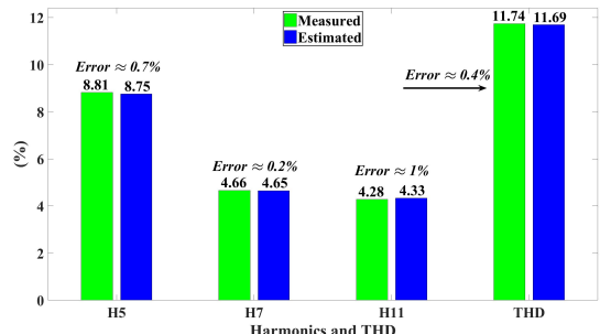
(b) Measured and estimated THD at the desired bus.
