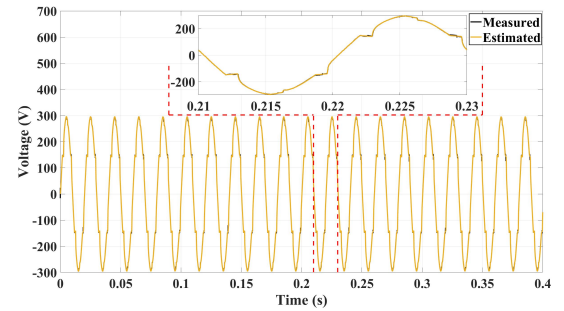
(a) Measured and estimated voltages of phase a at desired bus.
