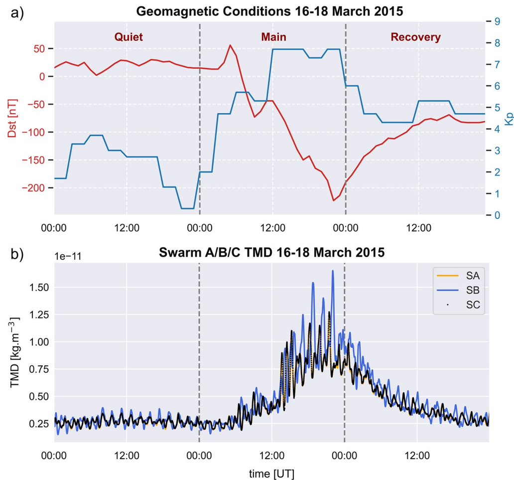
Fig. 1 St. Patrick's Day storm 2015. a geomagnetic activity represented by the Dst (red) and 3-h average Kp (blue) indices. b Along the orbit thermospheric mass density observations from Swarm-A, -B, and -C satellites (yellow, blue, and black) normalized to 400 km altitude. The period from 16 to 18 March 2015 includes a pre-storm quiet day, the main phase of the storm and the first day of the recovery phase. A strong perturbation in geomagnetic activity and neutral density is visible during the main phase of the storm
