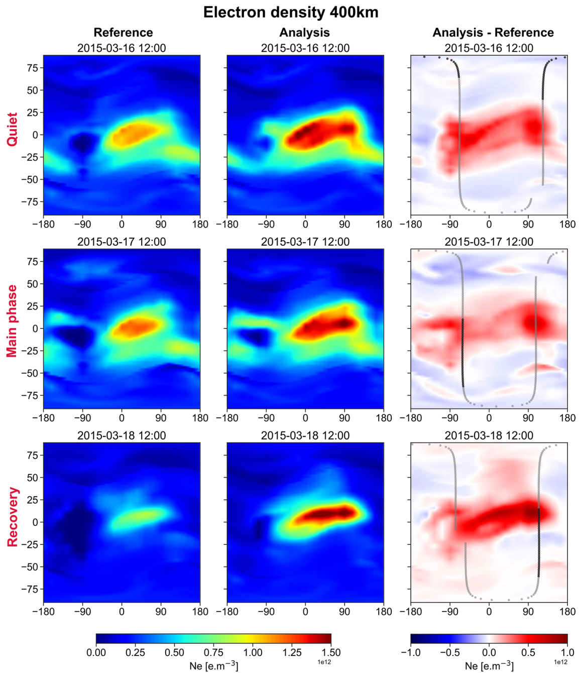
Fig. 4 Electron density maps at 400 km altitude for reference, analysis and analysis—reference difference at 1200 UTC (columns) during quiet, main phase and recovery days (rows). The location of Swarm-A orbit track is represented in the difference plot (grey line) with a highlighted area (black) of the last two assimilation intervals before 1200 UTC
