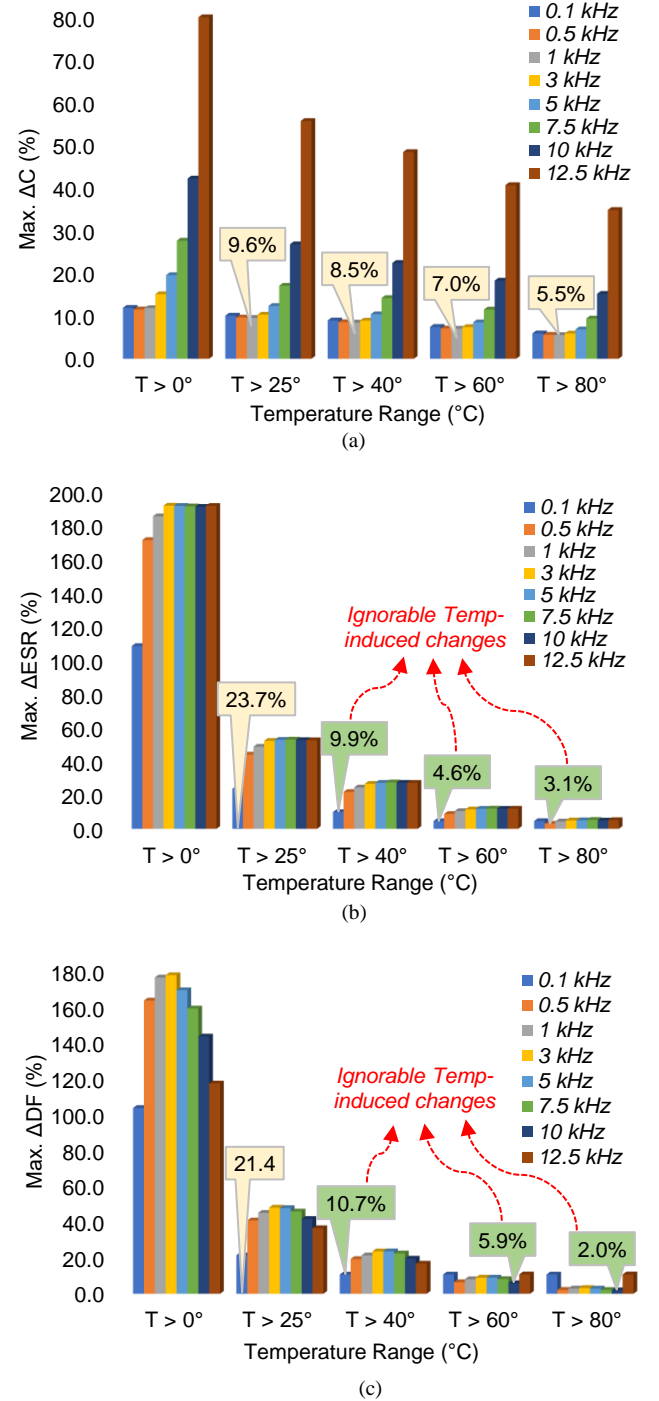
Fig. 9. Maximum temperature-induced changes in (a) capacitance, (b) ESR, and (c) DF for different temperature ranges (up to 160\text{ }^{\circ}\text{C} ) and frequencies.
