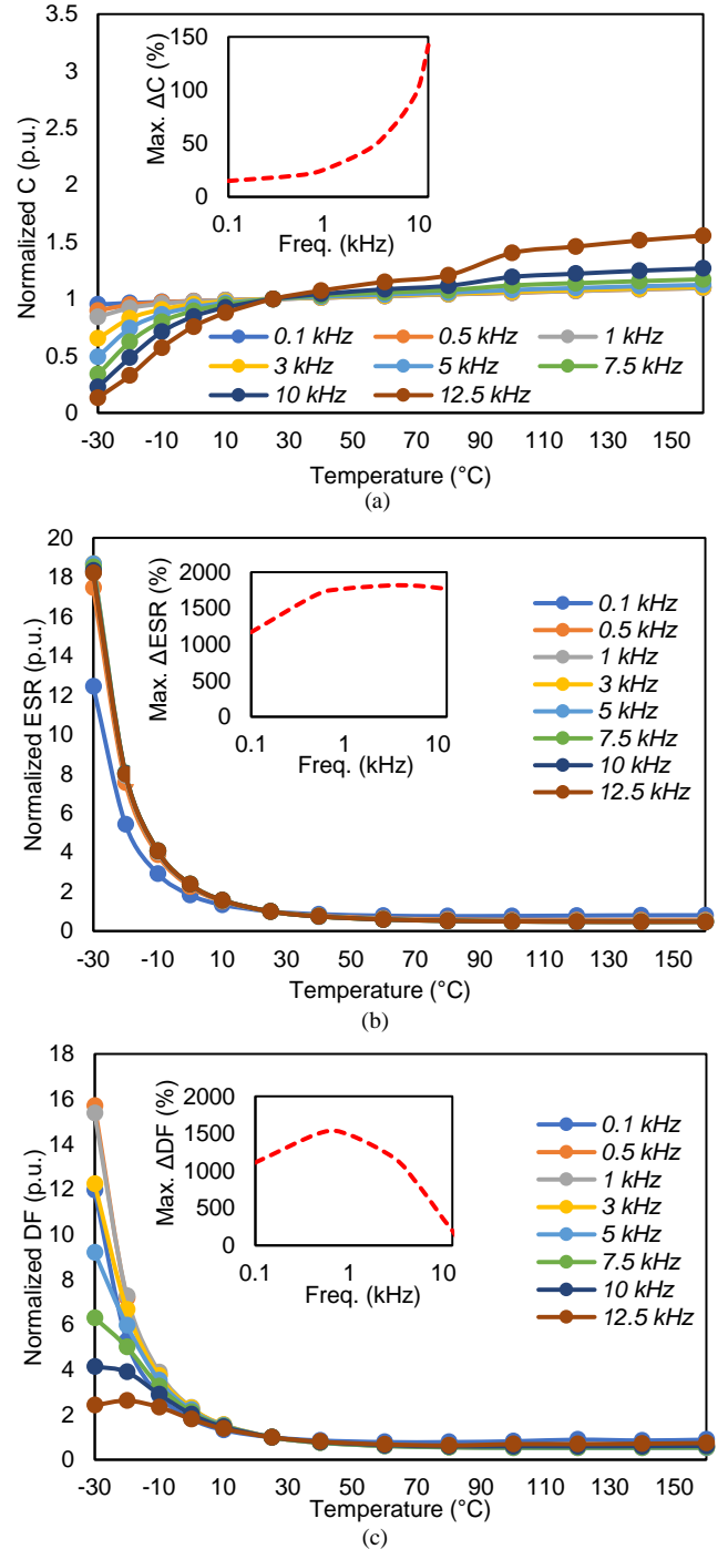
Fig. 8. Experimental results: Impact of temperature and frequency on the normalized values of (a) capacitance, (b) ESR, and (c) DF with respect to the values at 25 °C.
