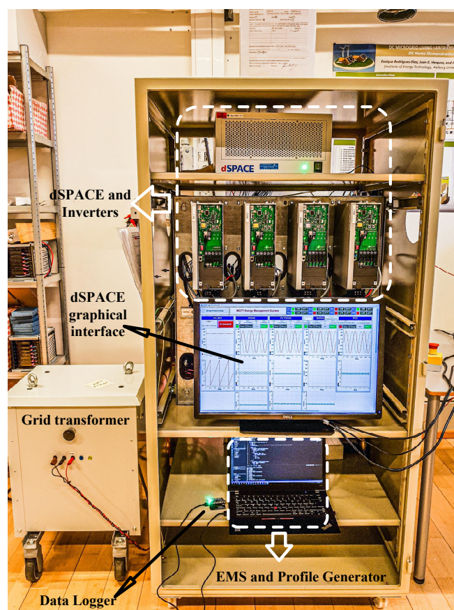
Figure 3. Experimental setup.
