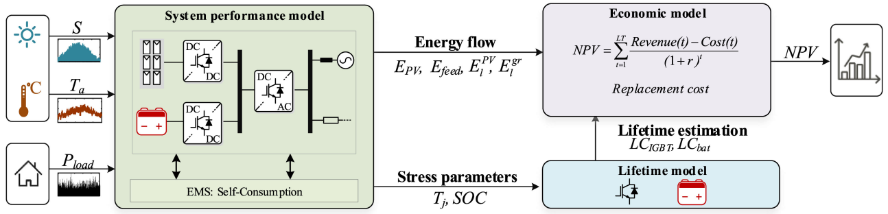
FIG. 1. PV-battery system model for the evaluation of the economic profitability influenced by the lifetime of the reliability-critical components. Model input are solar irradiance S , ambient temperature T_a , and load demand P_{load} . Model output is net present value NPV . SOC and LC_{bat} are battery state-of charge and lifetime consumption, respectively; T_j and LC_{IGBT} are switch junction temperature and lifetime consumption, respectively.
