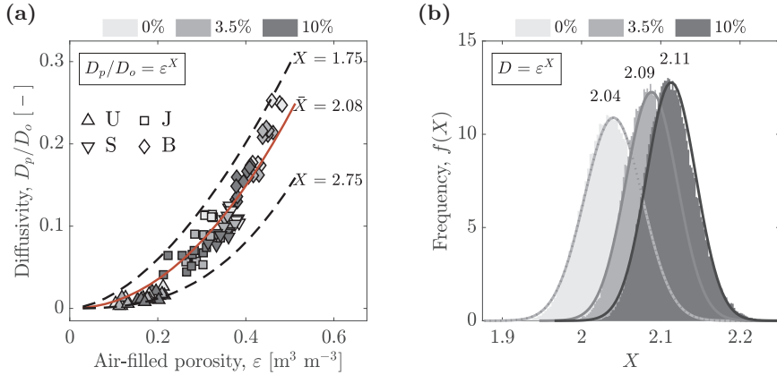
FIGURE 5: Relative diffusivity (a) as a function of the air-filled porosity ( \varepsilon ) and Equation 2 using X = \bar{X} = 2.08 (solid red line, see text); extrema (dashed lines, estimated by eye) and their respective X values; (b) result of the bootstrapped non-linear regression given as the frequency distributions of the fitted regression coefficients ( X ); mean X values for each GRF level are given above the distributions.
