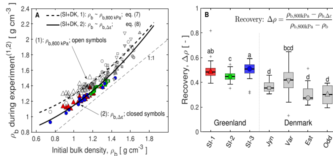
Fig. 8. Bulk density history at different stages (1 and 2) of the compression experiment. A : \rho_b at a normal stress of 800 kPa (1, open symbols; \rho_{b,800\text{kPa}} , \text{g cm}^{-3} ) and after the relaxation time (2, closed coloured symbols; \rho_{b,\Delta\epsilon} , \text{g cm}^{-3} ) as a function of \rho_b . The 1:1 line represents the initial \rho_b . Data reduced for better legibility (each third point). B : Recovery ( \Delta\rho , -), defined as the ability of a sample to return to its initial \rho_b during the relaxation time. Columns bearing the same letters are not statistically different on a 5% significance level. Greenland: \blacktriangle South-Igaliku 1 (SI-1), \blacksquare South-Igaliku 2 (SI-2), \bullet South-Igaliku 3 (SI-3); Denmark: \square Jyndevad (Jyn), \odot Estrup (Est), \nabla Varde (Var) and \triangle Odder (Odd).
