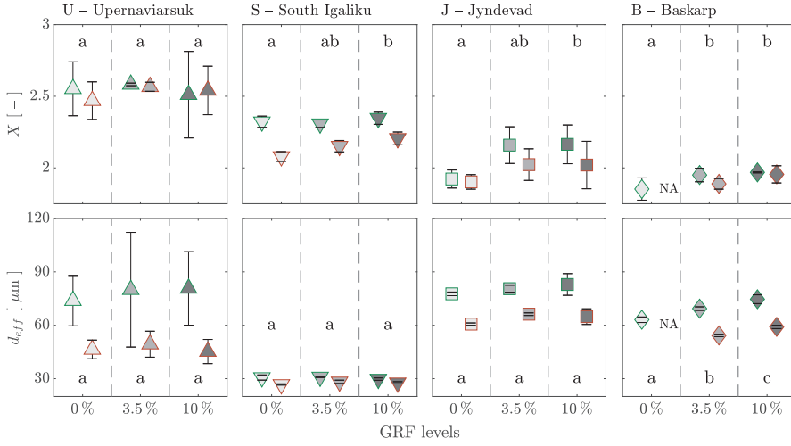
FIGURE 7: Pore network parameters at \psi = -300 hPa: X (upper plots) and d_{eff} (lower plots) before (left-hand symbol of each GRF level, green outline, bC) and after compression and rebound (right-hand symbol, red outline, aR). Symbols are mean values; error bars represent the standard deviation. Groups bearing the same letters were not statistically different from each other (each soil type was tested individually, bC and aR were combined).
