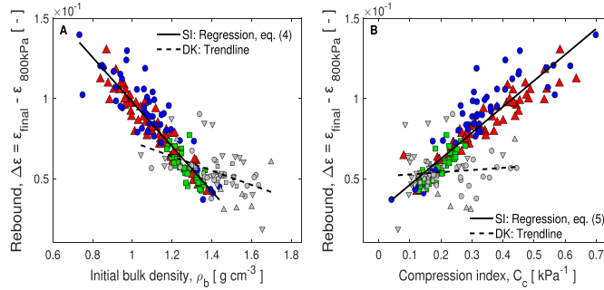
Fig. 7. The rebound ( \Delta\epsilon , -) expressed in terms of compressive strain as a measure of short term recovery from compaction. A : \Delta\epsilon as a function of the initial bulk density ( \rho_b , \text{g cm}^{-3} ) and the corresponding linear regression for the Greenlandic data (SI); the dashed line shows the general trend of the Danish dataset. B : \Delta\epsilon versus the compression index ( C_c , \text{kPa}^{-1} ) and a linear regression for the Greenlandic data (SI); the dashed line shows the trend for the Danish dataset. Greenland: \blacktriangle South-Igaliku 1 (SI-1), \blacksquare South-Igaliku 2 (SI-2), \bullet South-Igaliku 3 (SI-3); Denmark: \square Jyndevad (Jyn), \odot Estrup (Est), \nabla Varde (Var) and \triangle Odder (Odd).
