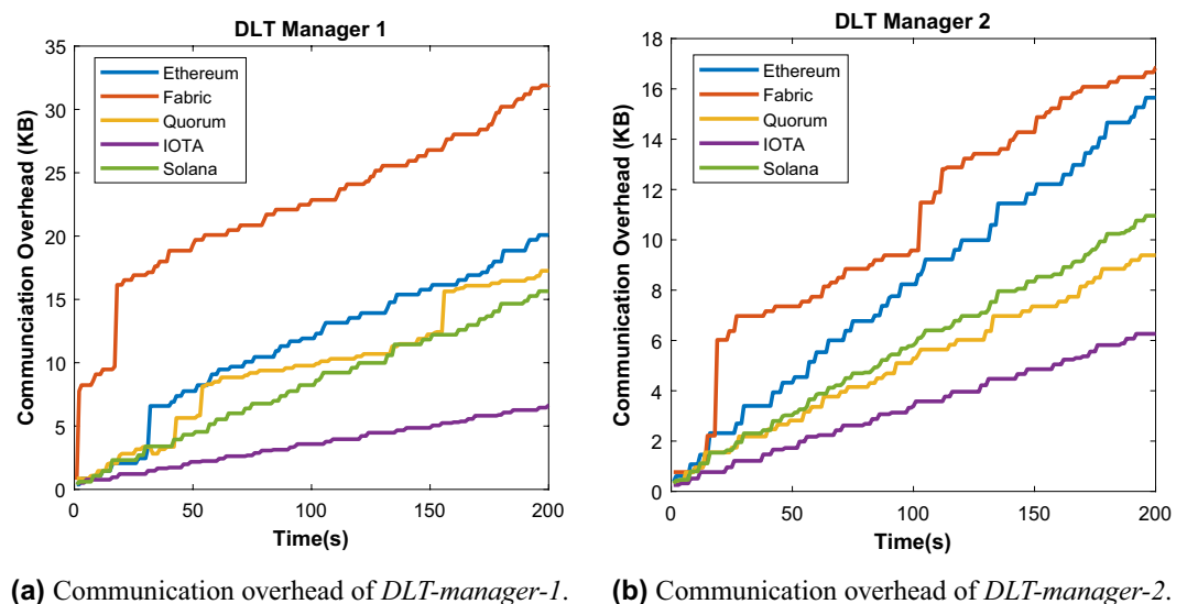
Figure 4. Communication overhead comparison of the 5 studied DLTs namely Ethereum, Hyperledger Fabric, IOTA, Quorum, and Solana.
