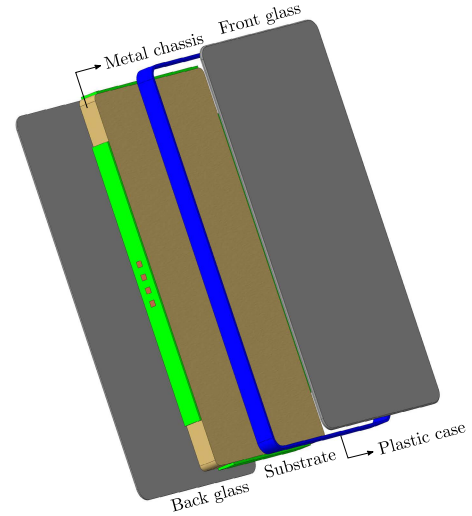
FIGURE 7. CST-modeled form factor.
