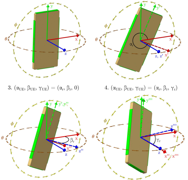
FIGURE 3. LCS (dotted axes) orientation with respect to the GCS (solid axes) through a sequence of 3 rotations: \alpha_r = \frac{11\pi}{6} , \beta_r = -\frac{\pi}{6} and \gamma_r = \frac{\pi}{6} .
