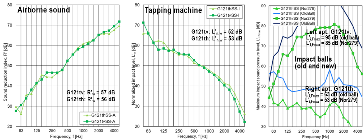
Figure 5 – Field measurement results for timber floor with additional ceiling, two apartments: (5a) Airborne sound insulation R' ; (5b) Impact sound level L'_{n,i} ; (5c) Impact balls L'_{i,Fmax}
