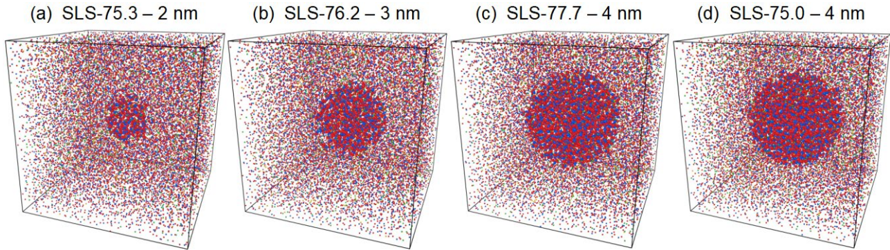
FIG. 3. Simulated structures of phase-separated soda-lime-silica (SLS) glasses with silica inclusions. The
