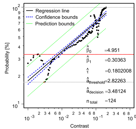
Figure 9. Regression analysis.
