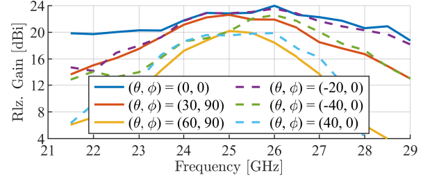
Fig. 10: Realized gain for different steering directions.
