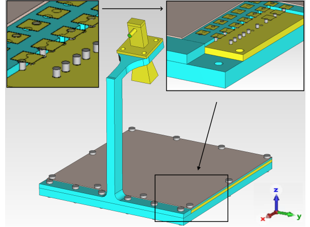
Fig. 7: Simulation model of the proposed reflectarray antenna.
