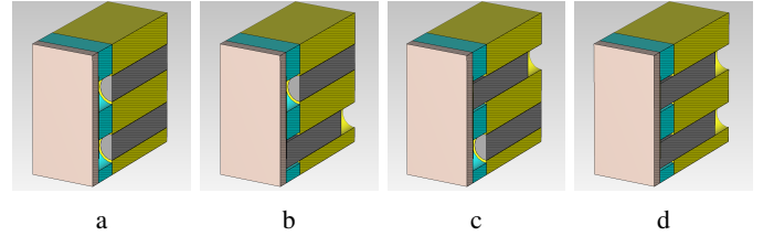
Fig. 3: The four stages of the prototype unit element. (a) State 00. (b) State 01. (c) State 10. (d) State 11.
