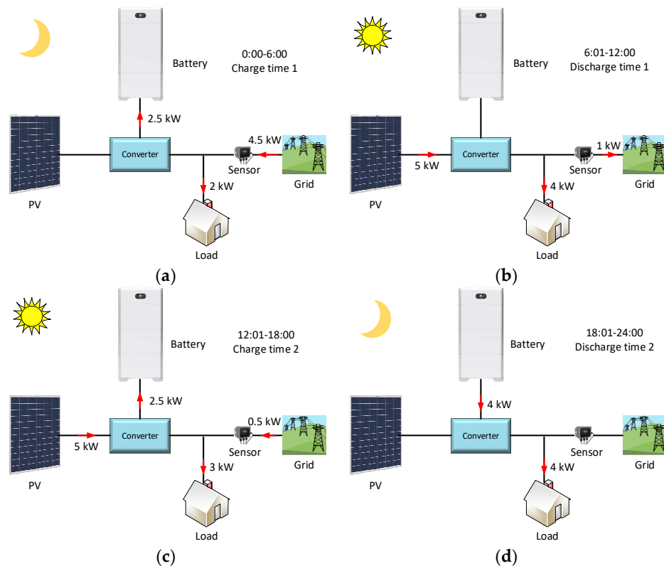
Figure 11. Examples of the time of use strategy.
