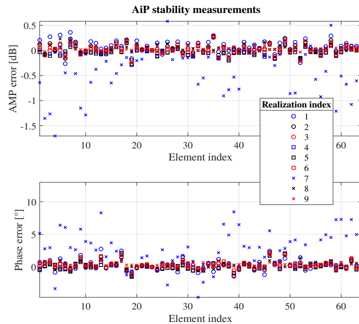
Figure 4. AiP elements stability measurement results.
