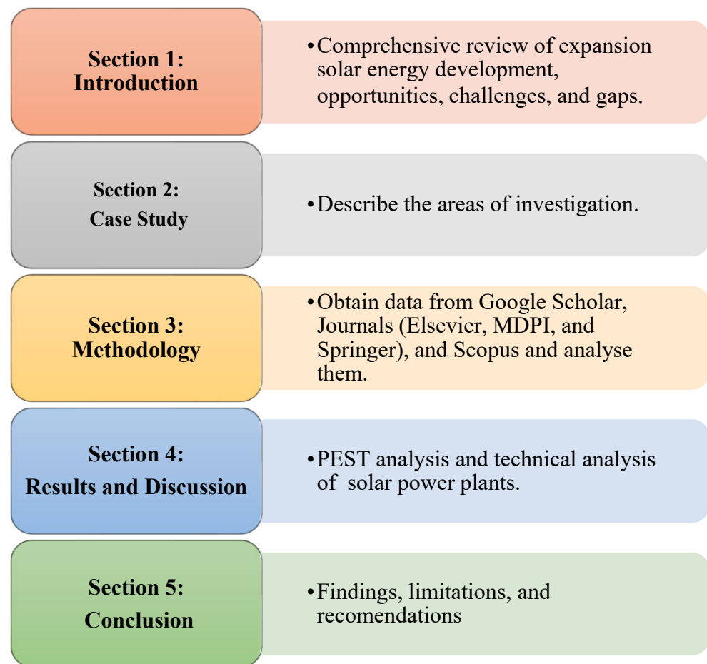
Figure 3. Research Methodology.
