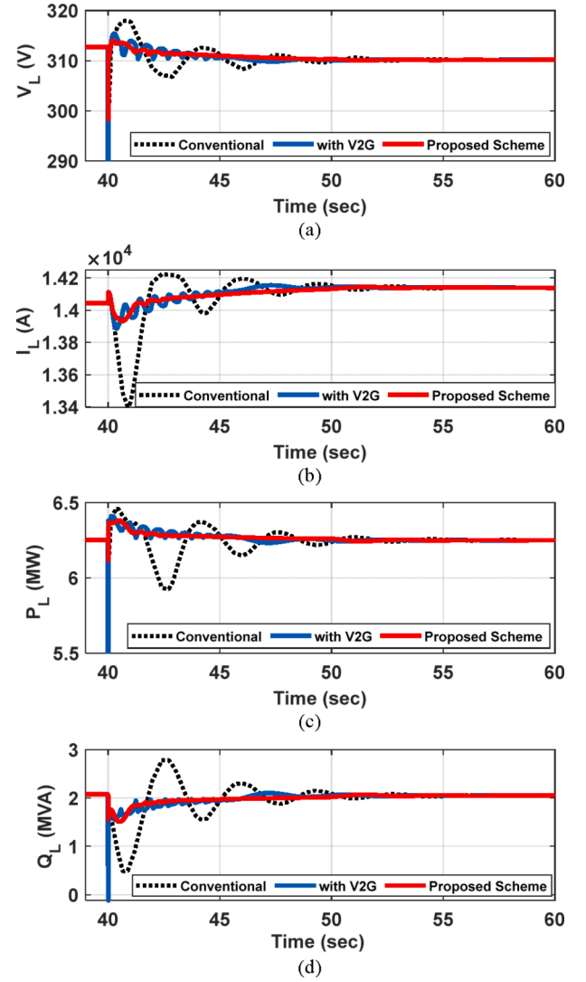
Fig. 12. Residential load responses: a) Voltage, b) current, c) active, d) and reactive power.
