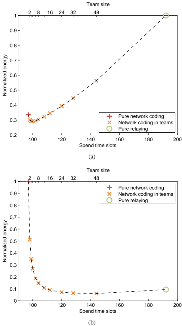
Fig. 5. Energy consumption versus transmission time for pure relaying, pure network coding and network coding in teams: (a) When WLAN power consumption is assumed and (b) when an ideal technology power consumption ( P_{idle} = 0 ) is assumed.
