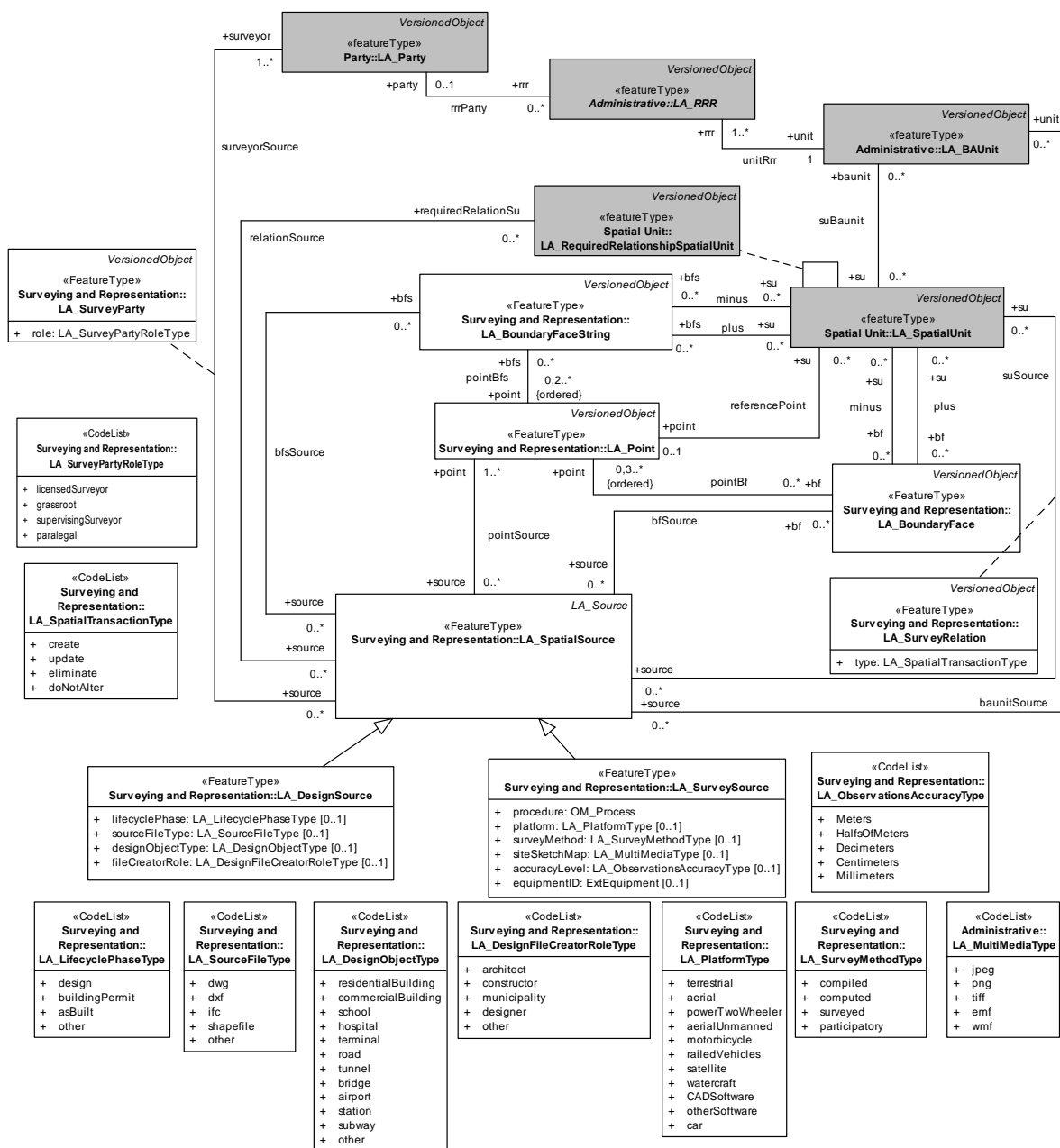
Figure 4. Basic Classes of Surveying and Representation Sub-package as submitted in CD of ISO19152-2 (2)
