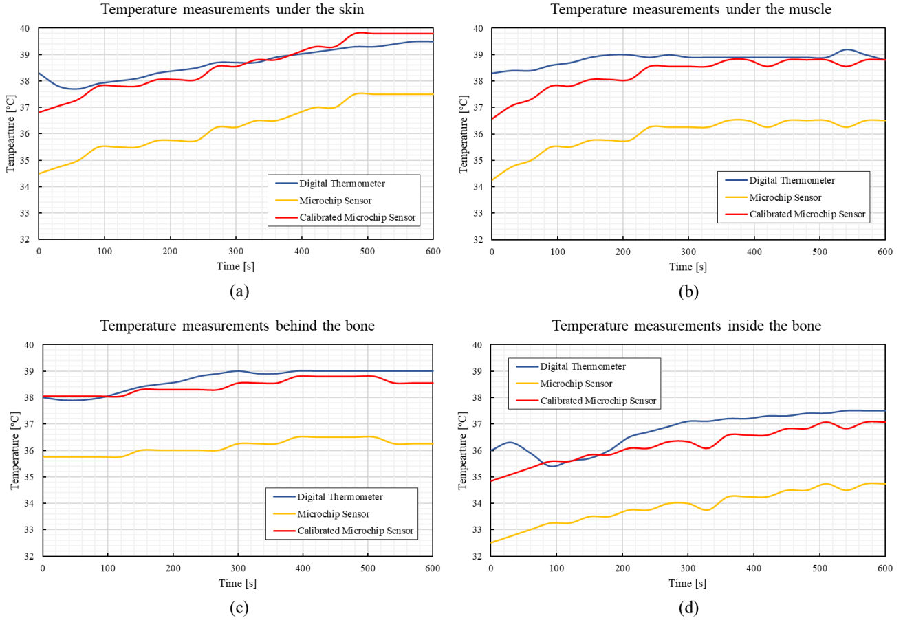
Fig. 6. Time-temperature results of the in-vivo test, measured by a digital thermometer and microchip sensor at different positions: (a) under the skin, (b) under the muscle, (c) behind the bone and (d) inside the bone.
