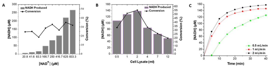
Fig. 1 Plot of [NADH] produced and % conversion in 5.7 mM hexanal as a function of (A) [\text{NAD}^+] at a flow rate of 2 \text{ ml min}^{-1} , (B) cell lysate loading; plot of [NADH] produced in 250 \mu\text{M NAD}^+ and a flow rate of 2 \text{ ml min}^{-1} (C) as a function of flow rate in 250 \mu\text{M NAD}^+ . Each determination was performed once for optimization purposes.
