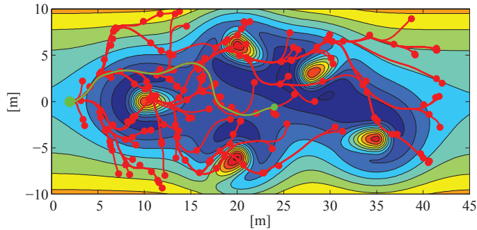
Fig. 12. An RRT for a robot starting at (2, 0) and the task of moving forward through the human populated environment. Only every 10th vertex is shown to avoid clutter of the graph. The vertices are the red dots, and the lines are the simulated trajectories. The green trajectory is the least cost trajectory.
