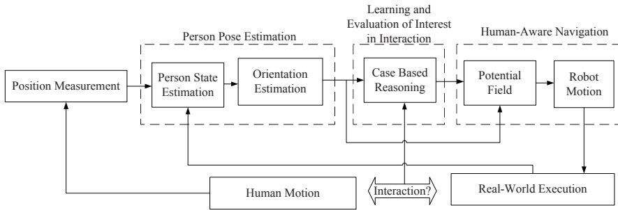
Fig. 1. An overview of how the different components are connected in the developed system. The three main parts engaged by the dashed squares.
