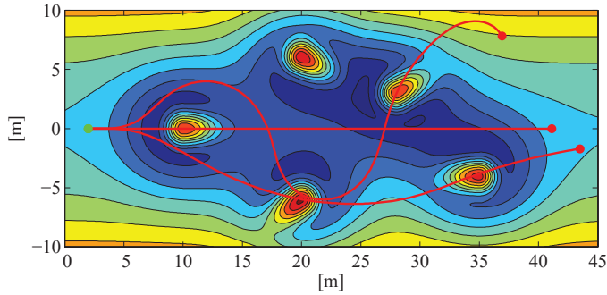
Fig. 5. Person landscape, which the robot has to move through. The robot starting point is the green dot at the point (2,0). Three examples of potential robot trajectories are shown. Even though it looks like the trajectories goes through the persons, this is not necessarily the case, since the persons might have moved, when the robot comes to the point.
