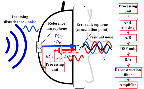
Fig. 1. Simplified modelling block diagram of FF ANC headphones with the extra delay D = ED_S + AD_S - AD_P in S(z) .
