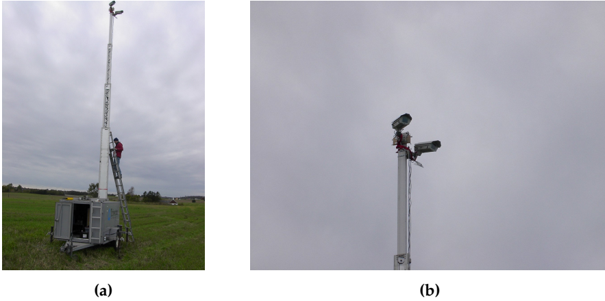
Fig. 2.7: (a) The Trivector Mobile mast setup in operation. (b) The Trivector Mobile mast with two installed cameras. Images provided by Aliaksei Lauresbyn, Lund University [1].
