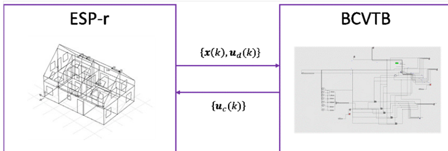
187 188 Fig. 1 Graphical representation of the communication architecture (measured state-disturbance 189 and window opening) of the coupled tools (ESP-r and BCVTB). 190
