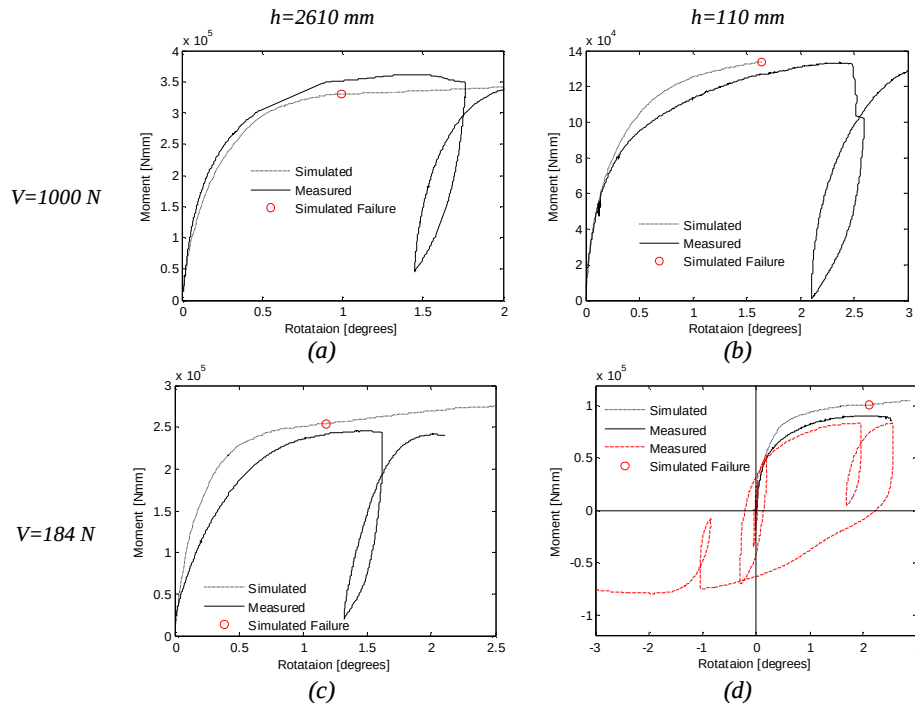
Figure 7.11 Simulation of selected laboratory tests. d/D=1
