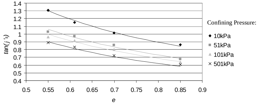
Figure 3.4 Relationship between the void ratio and \tan(j_s) from equation (3.2) (grey scale marks) at different confining pressures. The relationship suggested by Kerisel is shown for the respective stress levels by lines.
