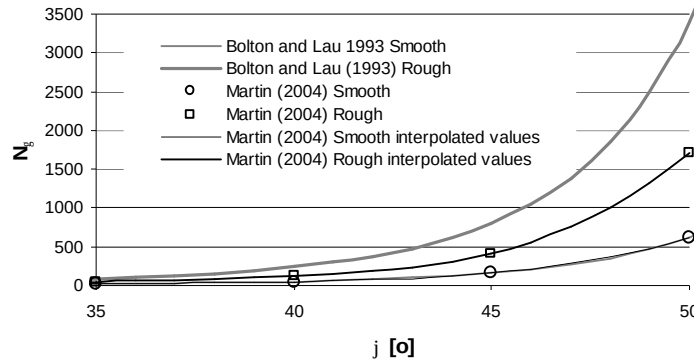
Figure 5.10 Values of the bearing capacity factor N_q for circular foundations.
