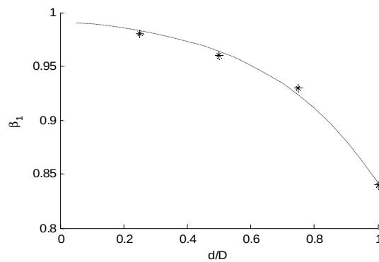
Figure 6.21 Calibrated values of b_1 using a tension capacity calculated with K_{tan}(d)=1 and m=2
