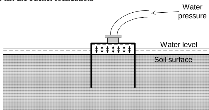
Figure 3.12 Removal procedure.
