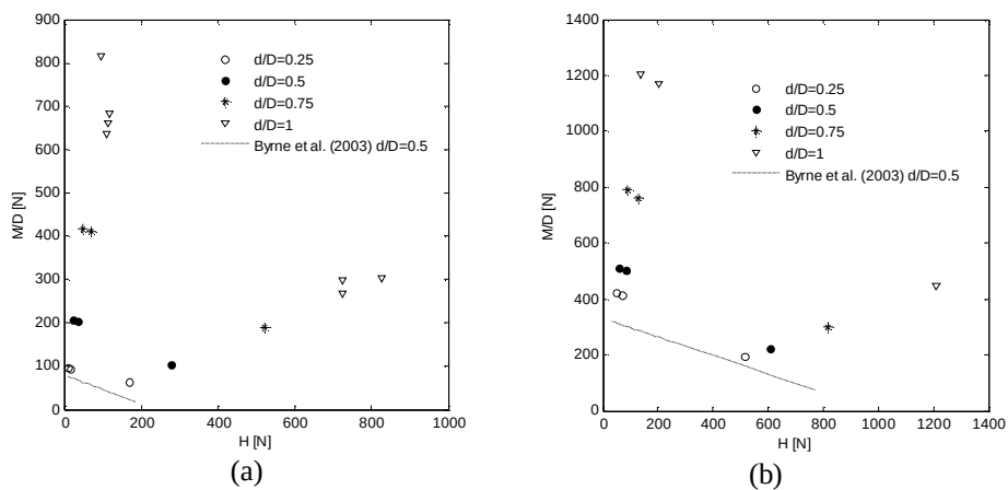
Figure 6.2 Failure values from tests with low V/V_{peak} values with a vertical constant load equal (a) V=184\text{N} , (b) V=1000\text{N} .
