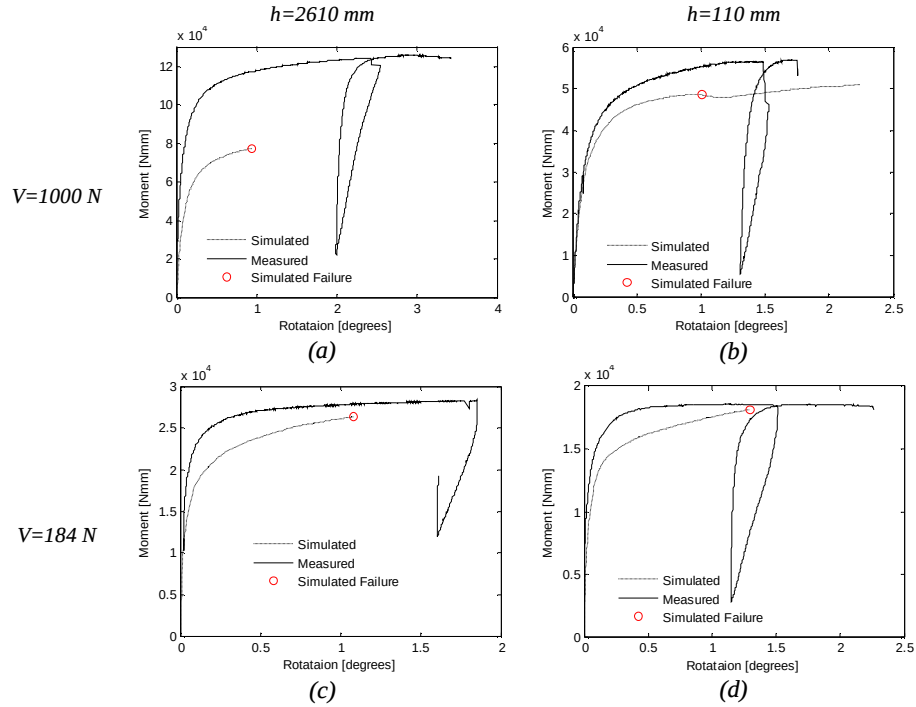
Figure 7.12 Simulation of selected laboratory tests. d/D=0.25
