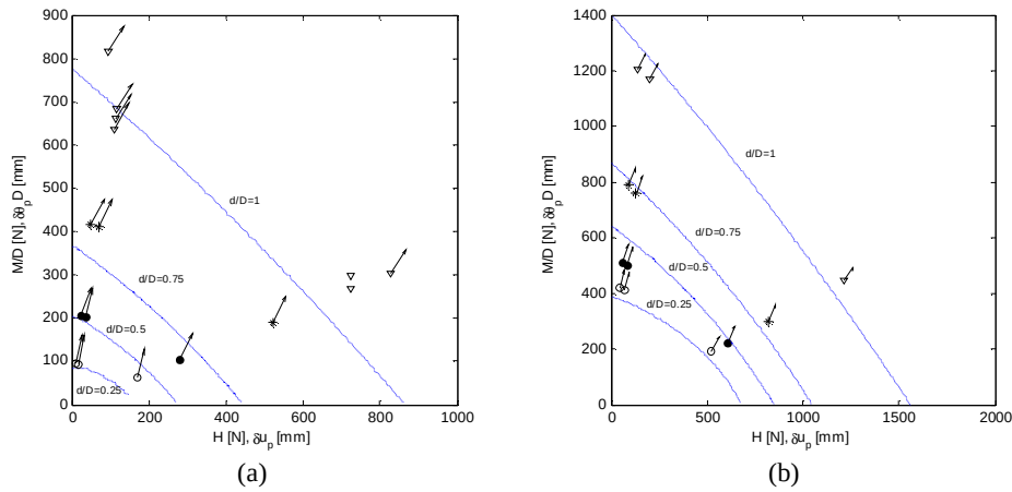
Figure 6.32 Direction of plastic increments at failure for tests performed with (a) V=184N and (b) V=1000N . The failure criteria are shown with parameters from Table 6.2, K_{tan}(b)=1 , m=2 and b_1 from Table 6.3.
