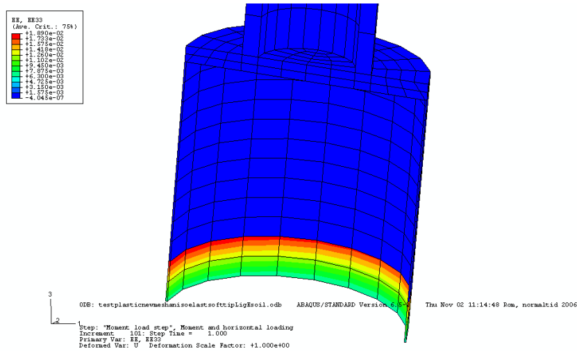
Figure D.8 Vertical strains in the bucket foundation at failure. E_{\text{skirt tip}} = E_{\text{soil}}
