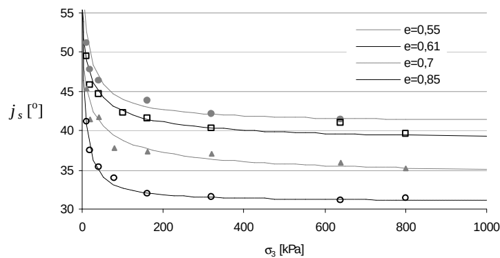
Figure 2.13 Variation of the triaxial secant friction angle for Aalborg University Sand No.0. The results from the triaxial tests are shown as points.
