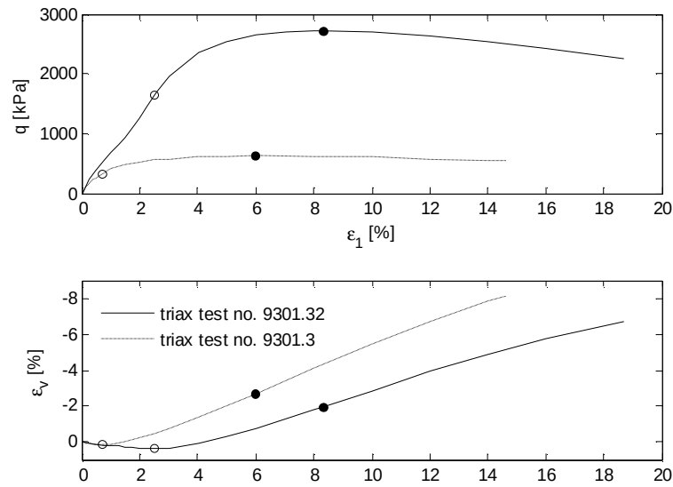
Figure 2.6 Triaxial results from tests on Aalborg University Sand No.0. Test 9301.3: Confining pressure=160kPa and Test 9301.32: Confining pressure=800 kPa. e = 0.61
