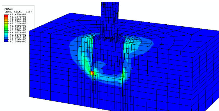
Figure 7.17 Magnitude of plastic strains at failure. V=1000\text{N} , d/D=1 and h=2610\text{mm} .
