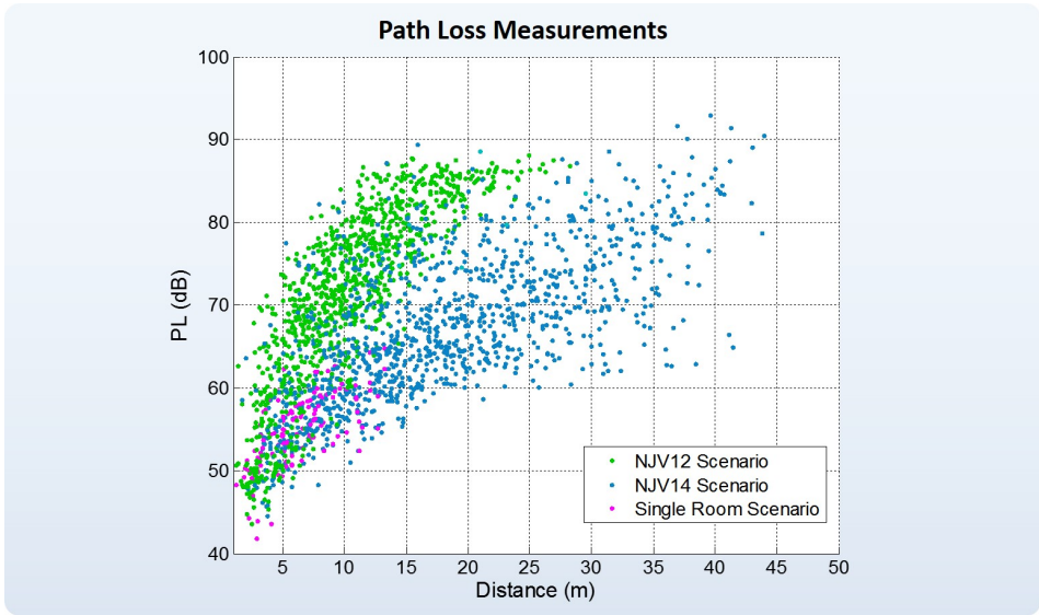
Fig. 5.2: Measured link path loss for the considered deployment scenarios.
