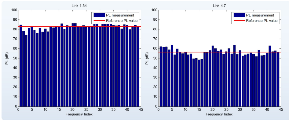
Fig. 5.3: Measured PL values in the NJV12 scenario for different carrier frequencies (i.e. 44 carriers from 4.91GHz to 5.89GHz). Values are shown for the link 1-34 (19.66 meters, 5 wall crossings) and link 4-7 (6.1 meters, LOS).
