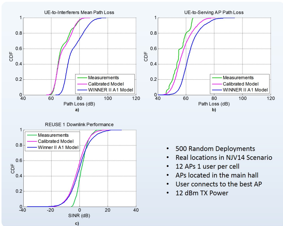
Fig. 5.10: Statistics related to 500 random network deployment in the NJV14 scenario.
