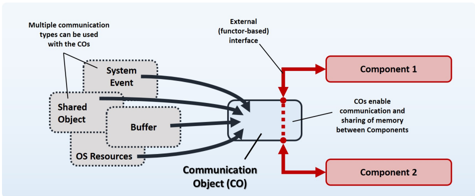
Fig. 3.7: Data communication by means of a Communication Object in ASGARD
