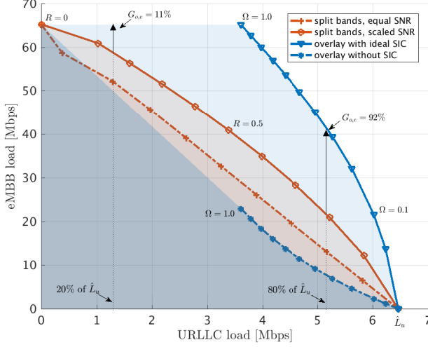
Fig. H.4: Achievable loads for URLLC and eMBB considering different receive strategies and moderate average SNR \gamma_u = 10 dB. W = 10 MHz, D = 256 bits, N_u = 50 , N_e = 2 and M = 4 .
