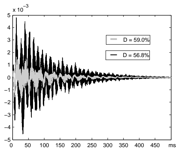
Fig. 24. Gray curves, the 25 impulse responses at the listening area in the Virtual Room before equalization. Black curves, after one point equalization. Loudspeaker setup .2.0
