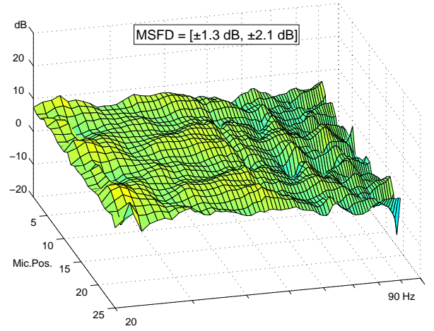
Fig. 47. Mean Sound Field Deviation ( MSFD ) of high pass filtered transfer functions at the listening area measured in the ITU Room. Upper setup .2.0. Lower after applying CABS .2.2. The loudspeaker response has been deconvolved.
