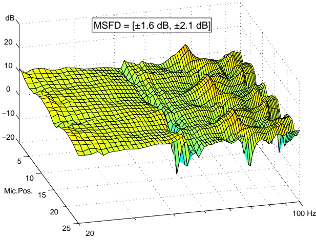
Fig. 46. Mean Sound Field Deviation ( MSFD ) of high pass filtered transfer functions at the listening area measured in the IEC Room. Upper setup .2.0. Lower after applying CABS .2.2. The loudspeaker response has been deconvolved.
