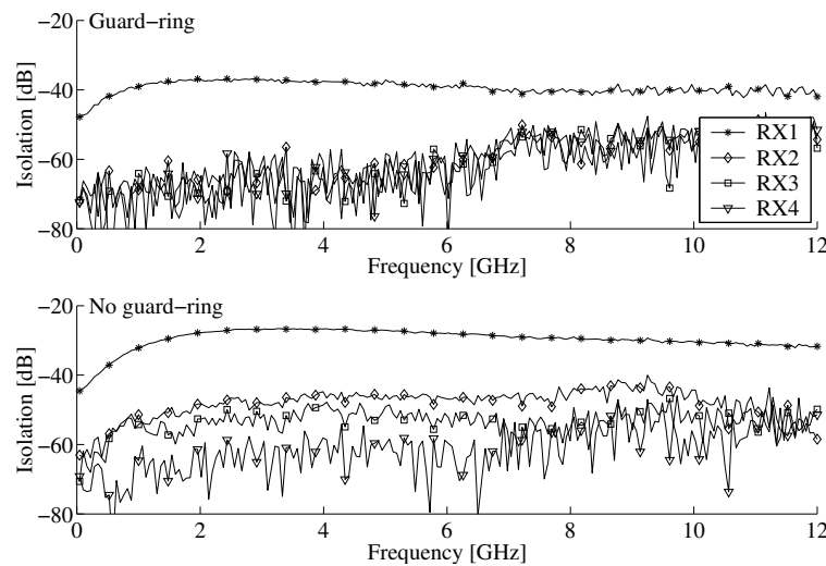
Figure 3.30: Measured isolation performance for structures with (top) and without (bottom) guard-rings where the test fixture ground-ring is cut.
