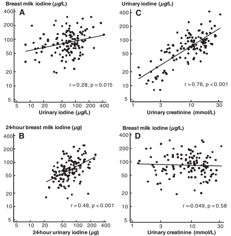
FIG. 3. Scatter plots of 127 samples illustrating the correlation between (A) maternal postpartum urinary iodine concentration and breast milk iodine concentration, (B) estimated 24-h breast milk iodine excretion and maternal postpartum 24-h urinary iodine excretion, (C) maternal postpartum urinary creatinine and urinary iodine concentrations, and (D) maternal postpartum urinary creatinine and breast milk iodine concentrations. All values were log-transformed for illustration and calculation of Pearson's correlation. Values on the axes are antilogged.
