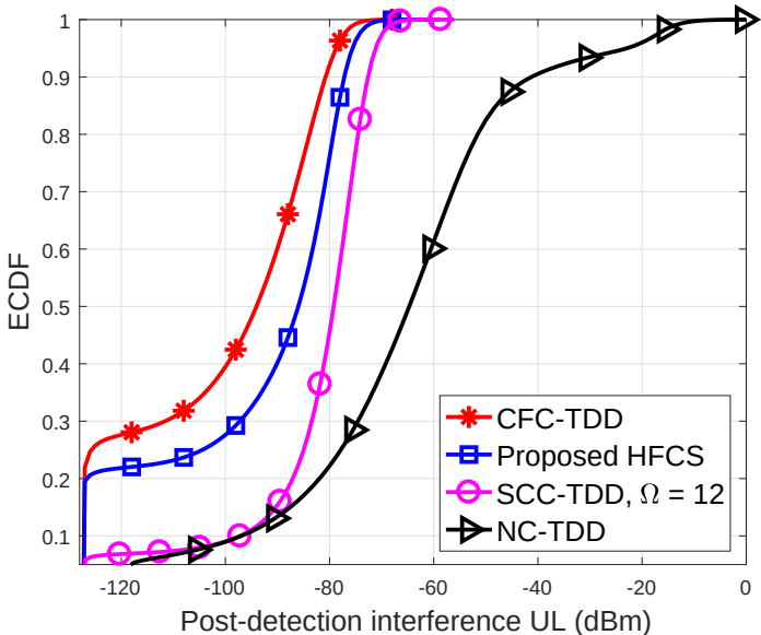
Fig. J.5. Post-receiver interference in UL direction (dBm).
