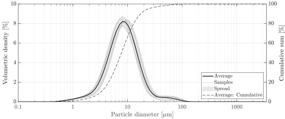
Fig. 3.4: Volumetric density function (left axis) and cumulative sum (right axis) of the untreated process water with soot particles.
