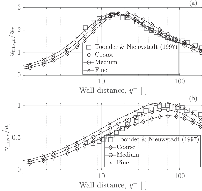
Fig. B.4: Normalised RMS velocity for the three mesh densities compared to experimental data of Toonder and Nieuwstadt (1997). The normalised axial RMS velocity, u_{rms,x}/u_{\tau} , is shown in Fig. B.4a and the normalised radial RMS velocity, u_{rms,r}/u_{\tau} , is shown in Fig. B.4b.
