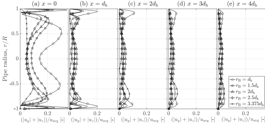
Fig. 4.5: Downstream normalised secondary velocity profile, (|u_y| + |u_z|)/u_{\text{avg}} , at x/d_h = 0 , x/d_h = 1 , x/d_h = 2 , x/d_h = 3 and x/d_h = 4 after the pipe bend.
