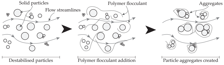
Fig. 1.8: Conceptual illustration of the flocculation process in a fluid flow. The polymer flocculant is added to the destabilised particles and due to the velocity fluctuations in the fluid, aggregates are created due to orthokinetic flocculation.
