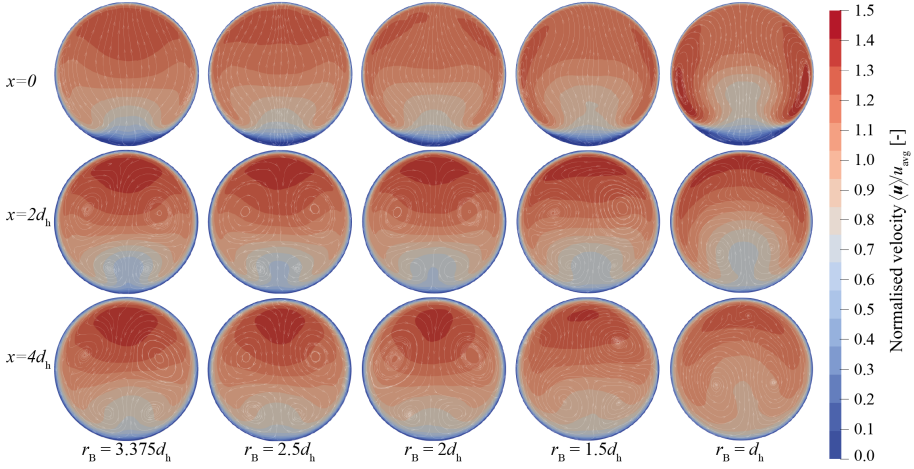
Fig. B.7: Normalised velocity, \langle u \rangle / u_{avg} , at lengths of x = 0 , x = 2d_h and x = 4d_h downstream of the bend for different bend radii. The secondary flows are visualised as streamlines.
