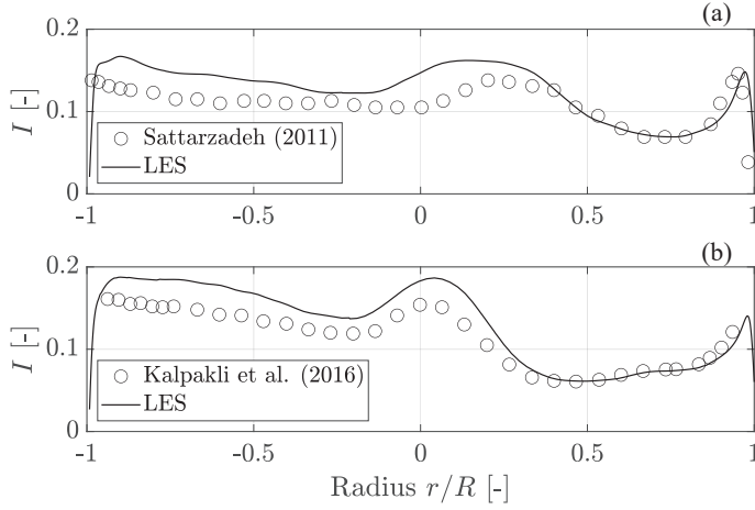
Fig. B.6: Turbulence intensity for a 90° bend with a fluid flow of Re = 14000 measured at a downstream location of x/d_h = 1.5 in Fig. B.6a and x/d_h = 0.67 in Fig. B.6b
