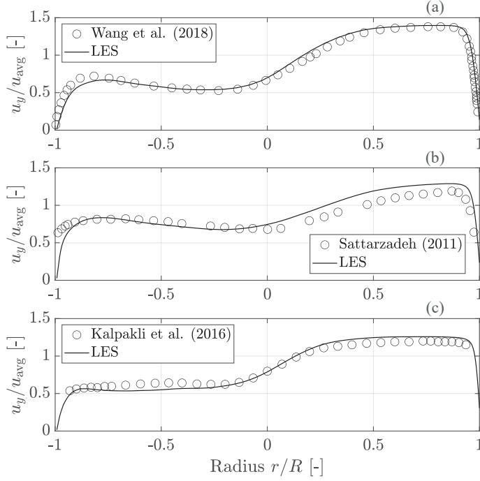
Fig. B.5: The normalised streamwise velocity, u_y/u_{avg} , for a pipe with a 90^\circ bend. The streamwise velocity for Re_d = 5300 and r_B = 1.25d_h are compared to the DNS data of Wang et al. (2018) in Fig. B.5a. The streamwise velocity for Re_d = 14000 and r_B = 1.58d_h is compared to PIV-HW data of Sattarzadeh (2011) Sattarzadeh (2011) and Kalpakli et al. (2016) Kalpakli Vester et al. (2016) measured at a downstream length of x/d_h = 1.5 in Fig. B.5b and at a downstream length of x/d_h = 0.67 in Fig. B.5c.
