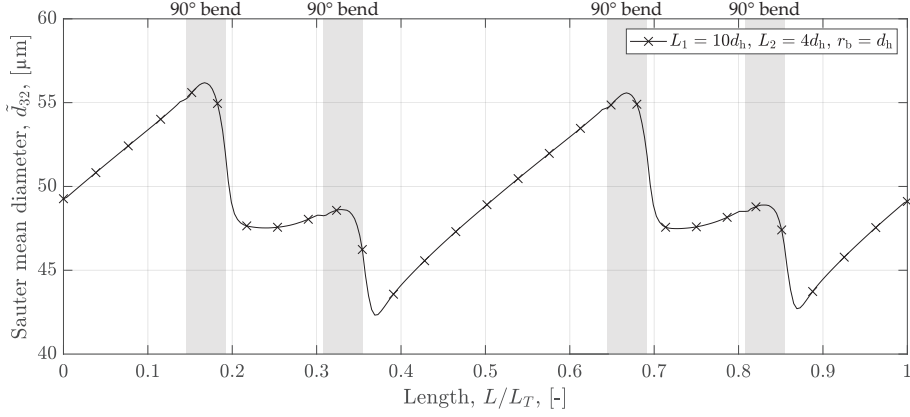
Fig. 4.8: Cross-sectional averaged Sauter mean diameter, \tilde{d}_{32} for a configuration.
