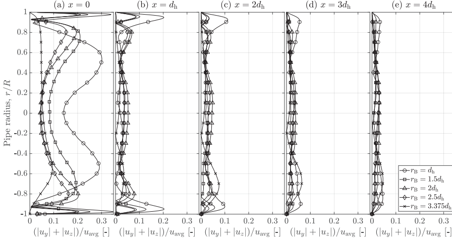
Fig. B.13: Normalised secondary velocity, (|u_y| + |u_z|)/u_{avg} , at B.13a: x = 0 after the pipe bend, B.13b: x = 1d_h after the pipe bend, B.13c: x = 2d_h after the pipe bend, B.13d: x = 3d_h after the pipe bend and B.13e: x = 4d_h after the pipe bend.
