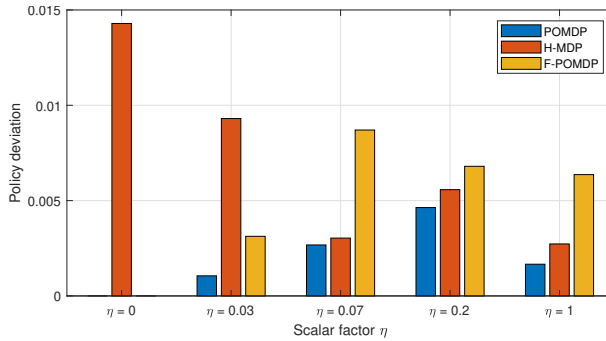
Fig. D.9: The deviation from the optimal MDP policy of full observably.
