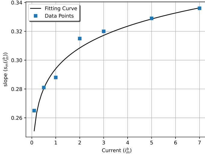
Fig. G.4: Variation of battery discharge slope for different discharge current.
