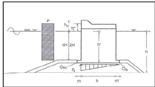
Fig. 13. Example of wave pressure distribution at a vertical face breakwater
