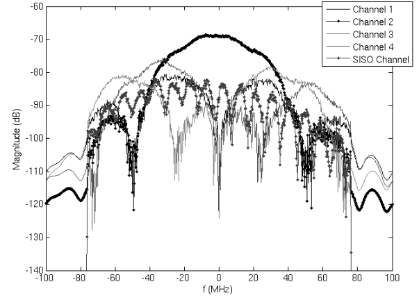
Fig. 13. Example case of the open channel with added frequency selectivity using different antenna phase topologies with the impact of a passing vehicle
