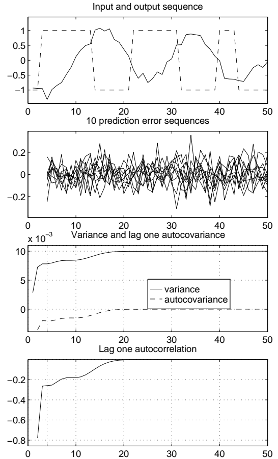
Figure 6: Residual properties for the third order system with damping factor 0.5 (BC method).
