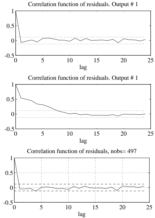
Figure 9: Autocorrelation tests corresponding to the three sequences shown in Fig. 8.
