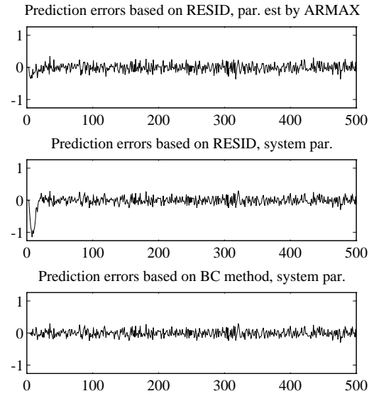
Figure 8: Prediction error/residual sequences from the same input/output sequence.
