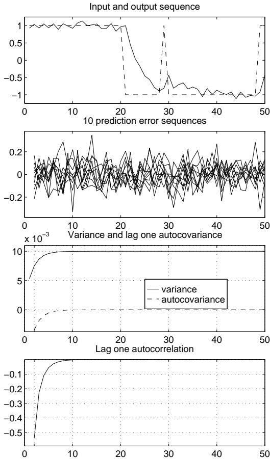
Figure 5: Residual properties for the first order example (BC method). t_s is marked with an extra tick-mark.
