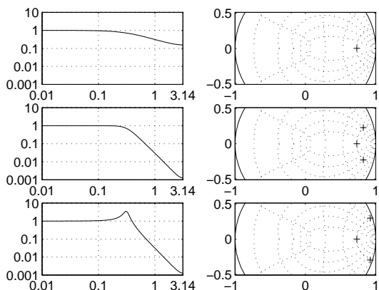
Figure 1: Gain and poles for the examples.
