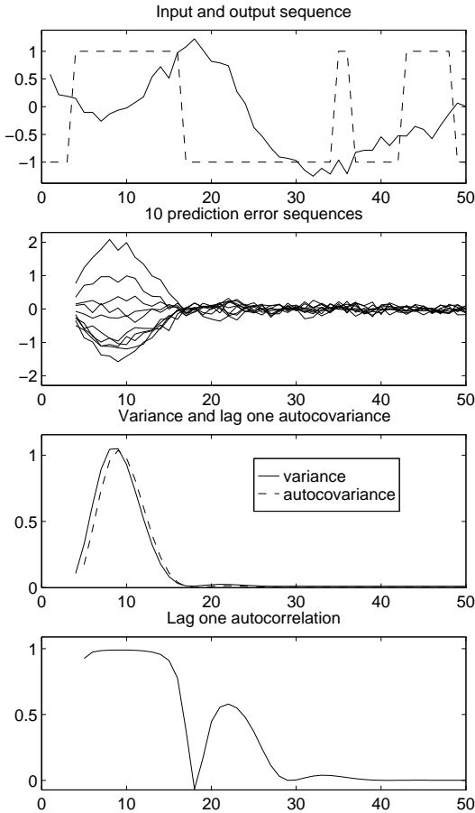
Figure 3: Prediction error properties for the third order system with damping factor 0.5 (DS method).
