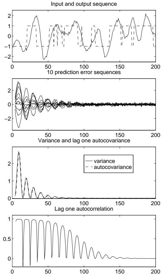
Figure 4: Prediction error properties for the third order system with damping factor 0.1 (DS method).
