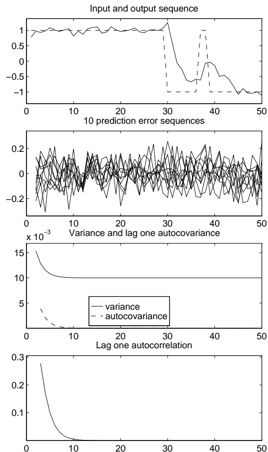
Figure 2: Prediction error properties for the first order example (DS method).
