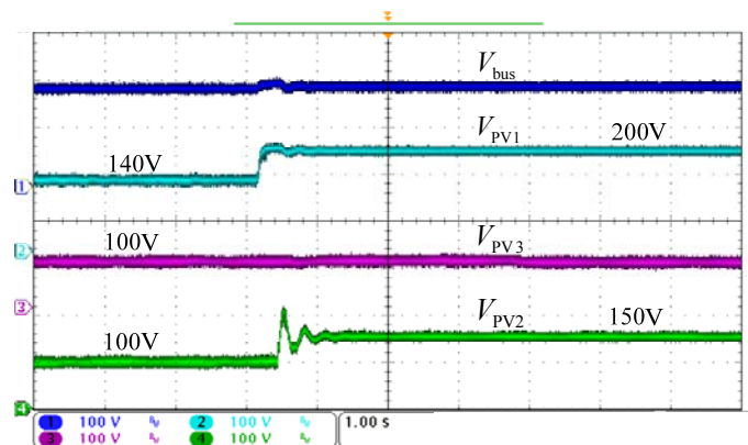
a. Dynamic response at load power decrease
