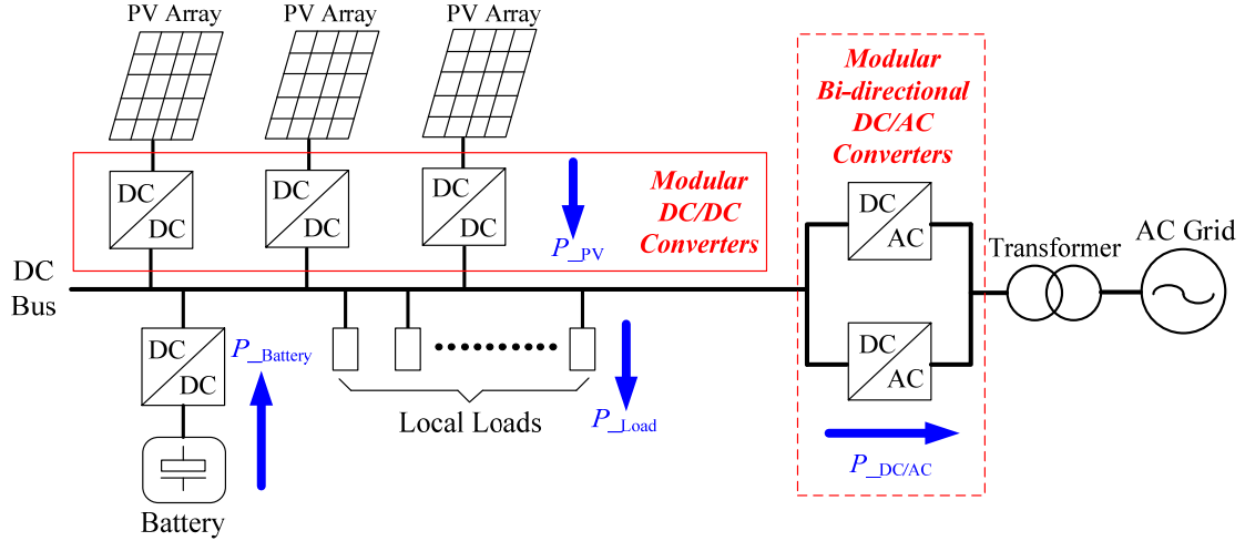
Fig.2 The DC bus based modular PV generation system
