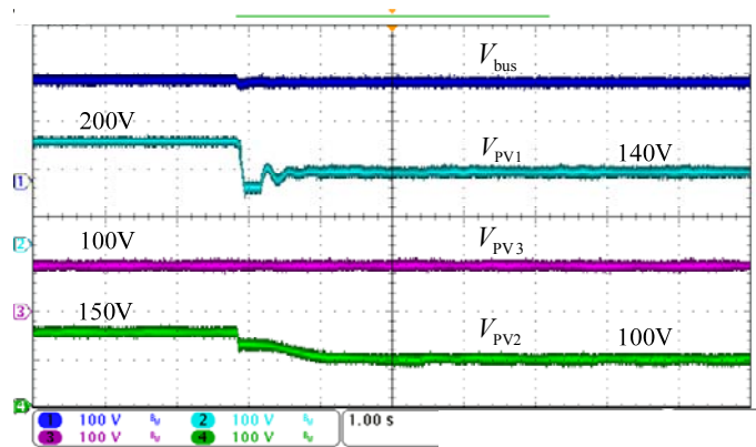
b. Dynamic response at load power increase
