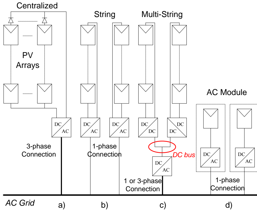
Fig.1 Configurations of PV generation systems
