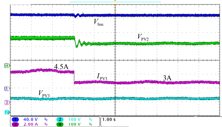
b. Dynamic response at PV power decrease
