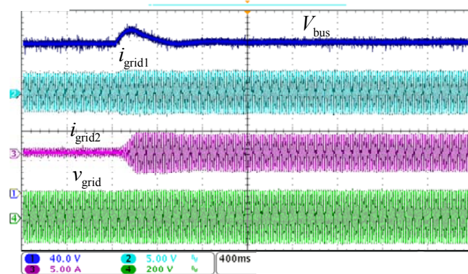
b. Dynamic response at load power decrease
