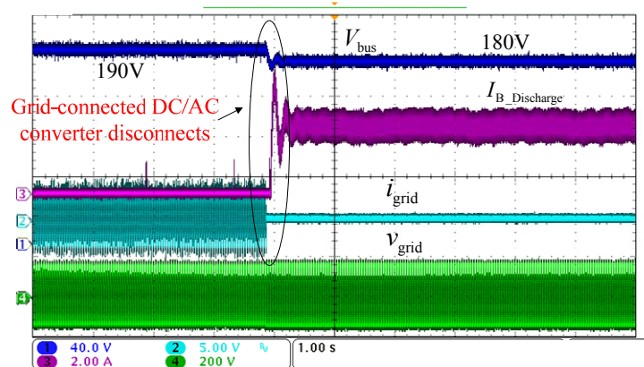
Fig.16 Experimental results in the transition from Mode II to Mode I
