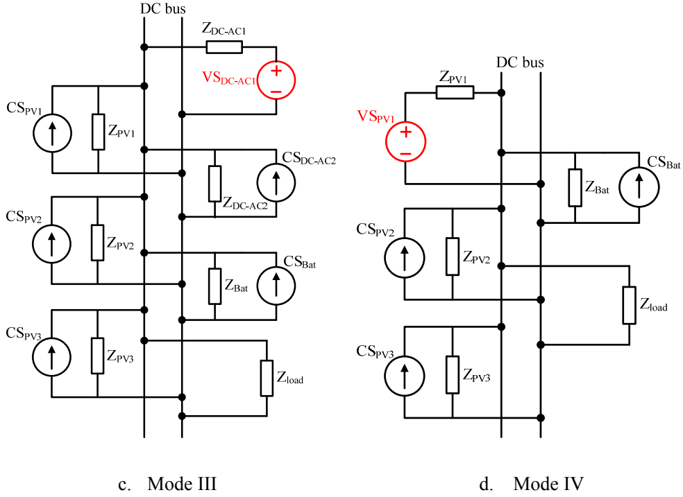
Fig.4 Equivalent circuits of the system under different modes
