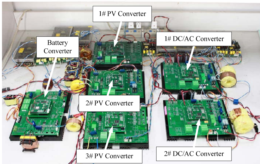
Fig.10 Photo of the experimental setup
