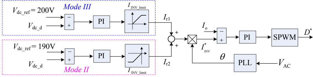
Fig.7 Local control diagram of grid-connected DC/AC converter
