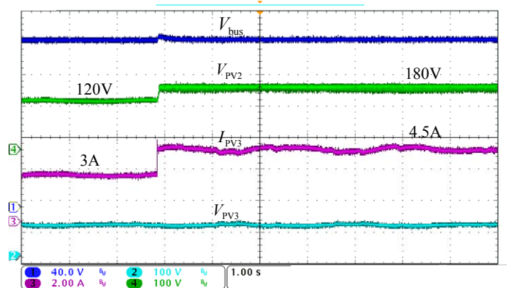
a. Dynamic response at PV power increase
