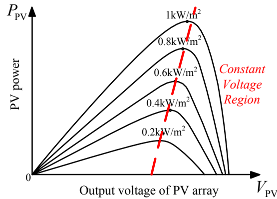
Fig.6 P-V curve of PV array
