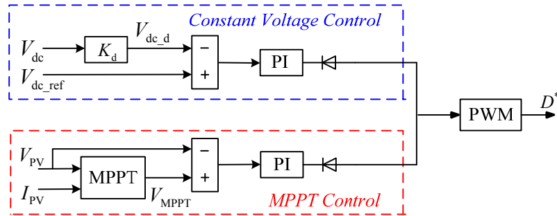
Fig.5 Control diagram of each modular DC/DC converter for PV array
