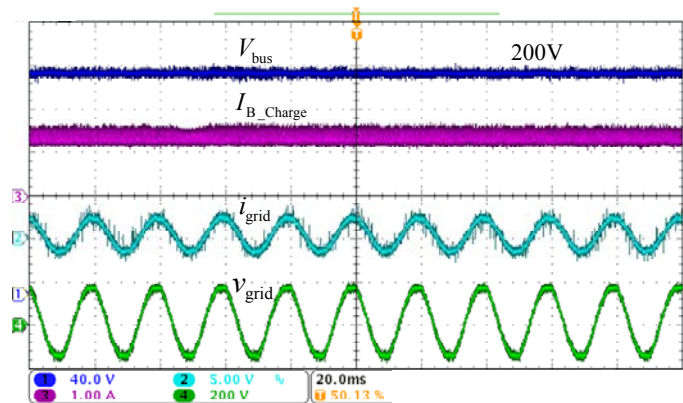
Fig.18 Steady-state experimental results in Mode III
