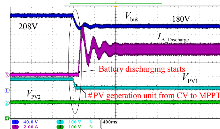
Fig.26 Experimental results in the transition from Mode IV to Mode I
