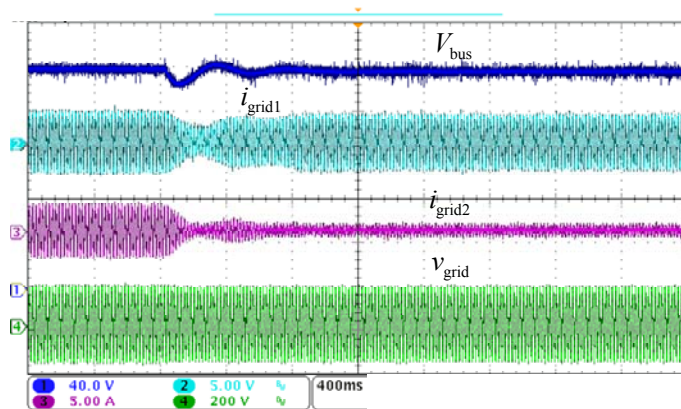
a. Dynamic response at load power increase
