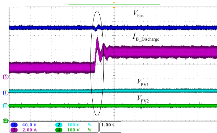
a. Dynamic response at load power increase
