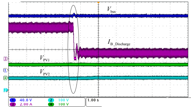
b. Dynamic response at load power decrease
