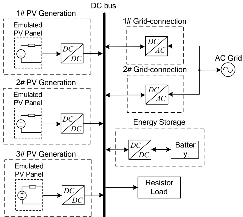
Fig.9 Configuration of the experimental setup
