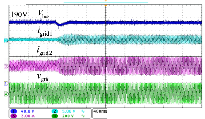
a. Dynamic response at load power increase
