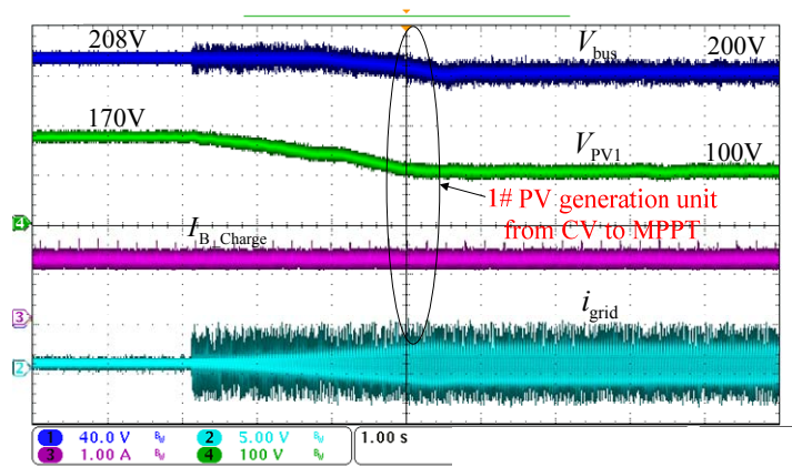
Fig.23 Experimental results in the transition from Mode IV to Mode III
