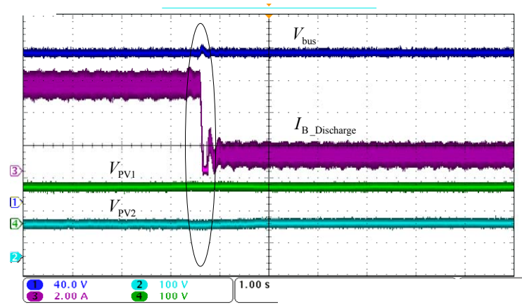
b. Dynamic response at load power decrease
