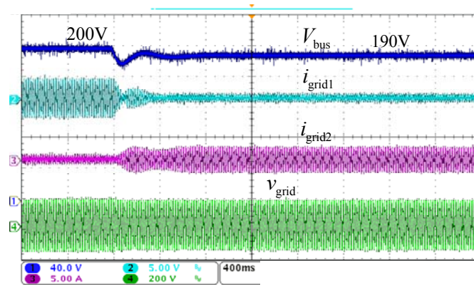
Fig.21 Experimental results in the transition from Mode III to Mode II with two DC/AC converters
