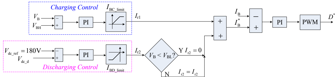
Fig.8 Control diagram of DC/DC converter for battery
