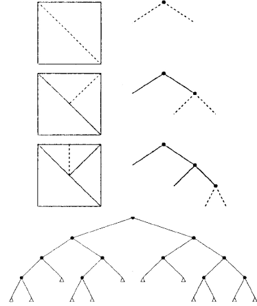
Figure 1: An illustration of building BTree using BTTC. The last figure shows an example of a final BTree.
