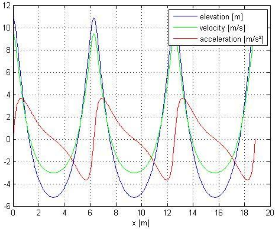
Wave profile for [Hmax=16,1m ; T=10,6s]
