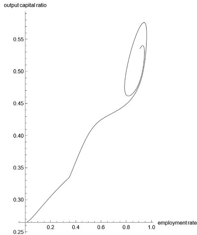
Fig. 1c. Simulation of baseline model with divergence (investment parameter = 1.08).
