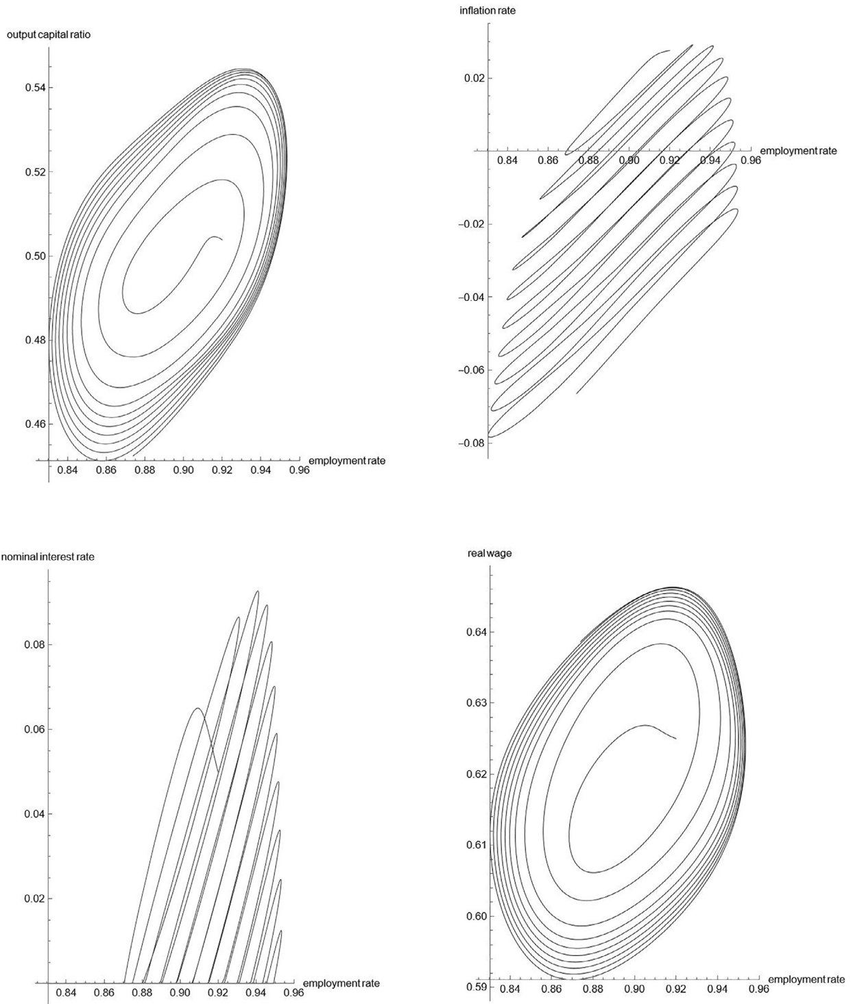
Fig. 5. Extended model with large investment parameter ( \rho_1 = 1.2 ).
