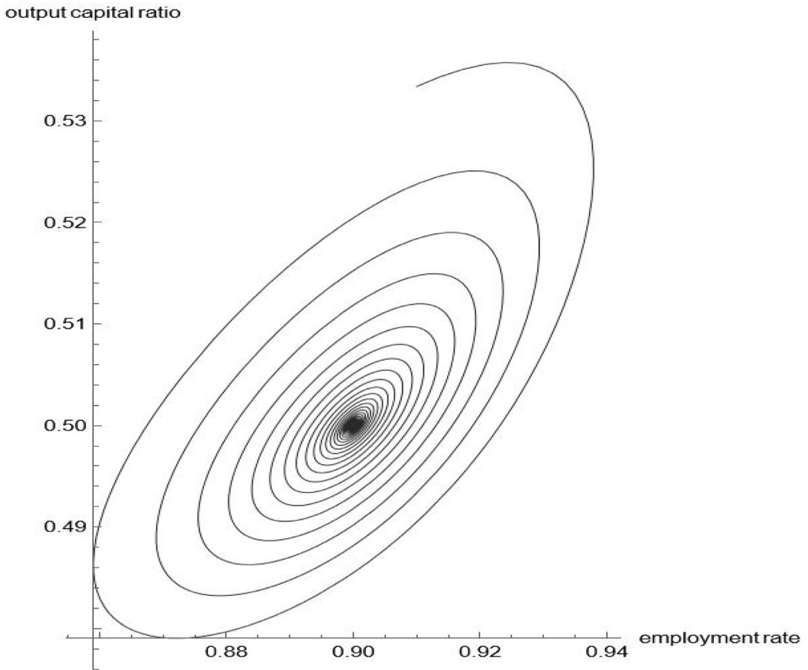
Fig. 1b. Simulation of baseline model with local stability (investment parameter = 0.97).
