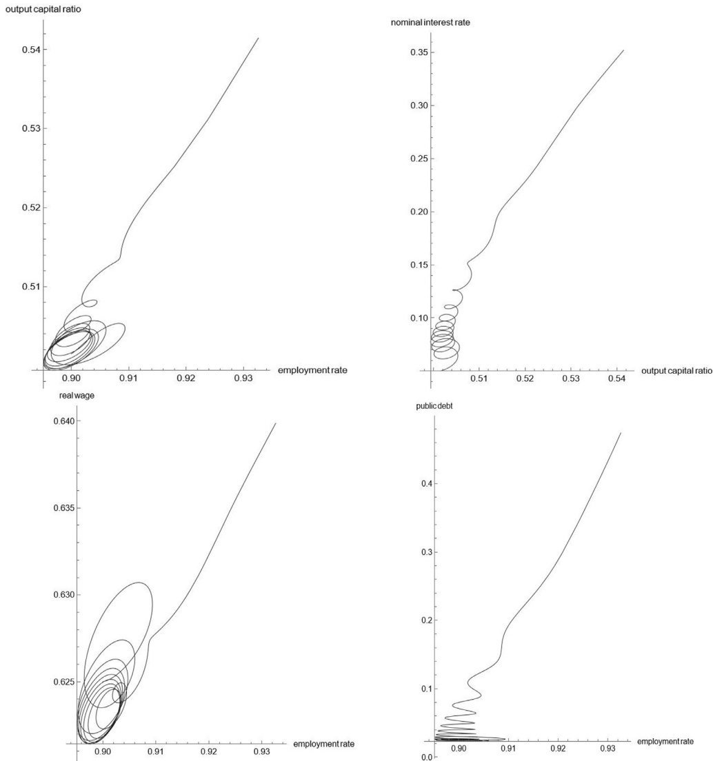
Fig. 4. Extended model without feedback from government debt ( \gamma_4 = 0 ).
