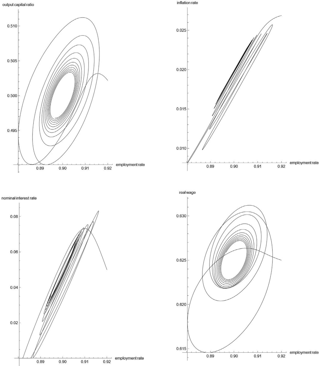
Fig. 7. Extended model with large investment parameter and induced changes of fiscal and monetary policy ( \rho_1 = 1.2, t_2 = 0.1, \gamma_3 = 200, \alpha_r = 3, \theta_1 = 4 ).
