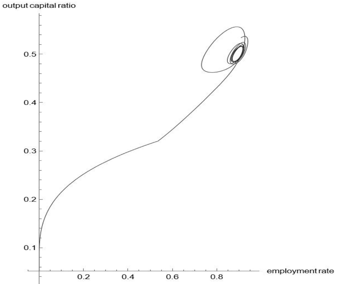
Fig. 2a. Simulation of baseline model with endogenous wage growth ( \alpha_1 = 0.01, \alpha_2 = 0 ).
