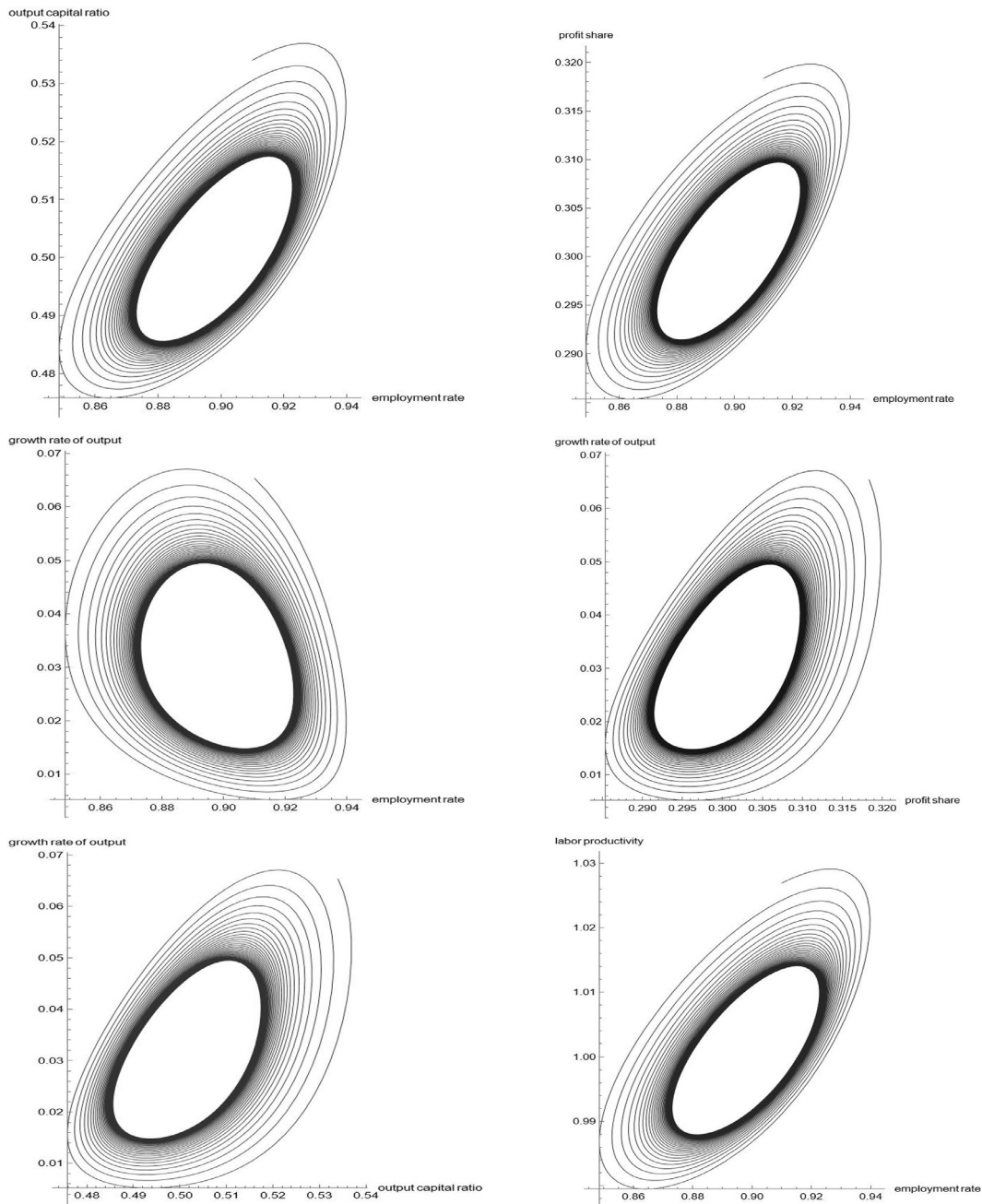
Fig. 1a. Limit cycle in simulation of baseline model (investment parameter = 1).
