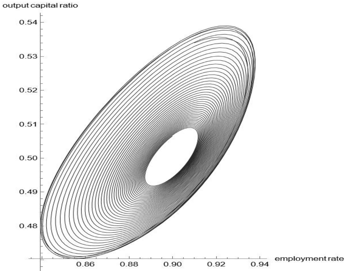
Fig. 2b. Simulation of baseline model with endogenous wage growth ( \alpha_1 = 0, \alpha_2 = 0.1 ).
