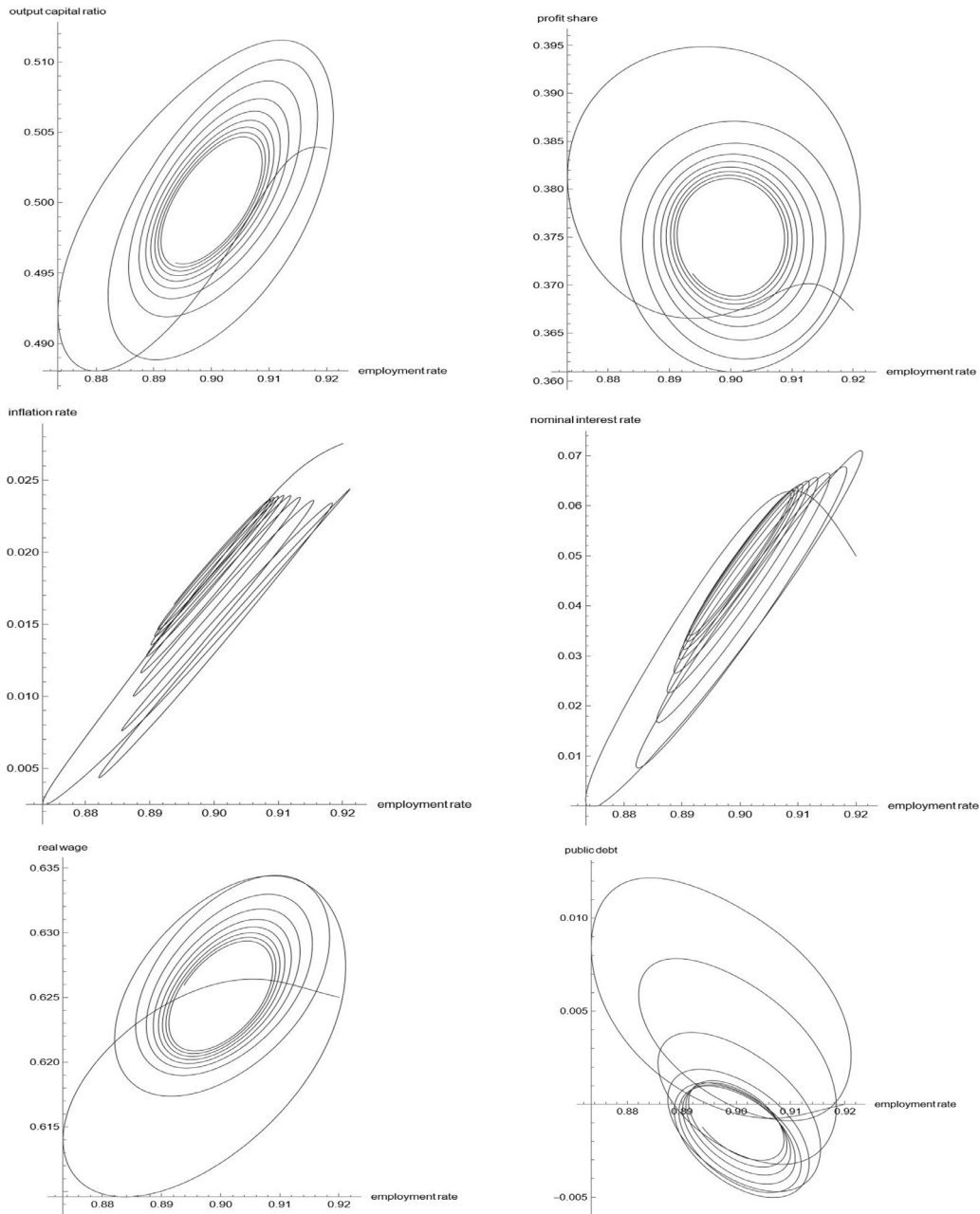
Fig. 3. Extended model with slow convergence ( \rho_1 = 0.89 ).
